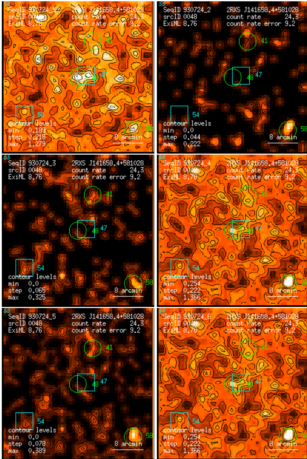
Figure 48: RASS 930724: detection 0048: band rate images, Gaussian filter: (1) PSPC channels 11 – 41, (2) 52 – 90, (3) 91 – 201, (4) 11 – 235, (5) 52 – 201, (6) 11 – 201. Broad band rates in counts/ks. Band rate contour levels in counts/ks/arcmin 2 .
