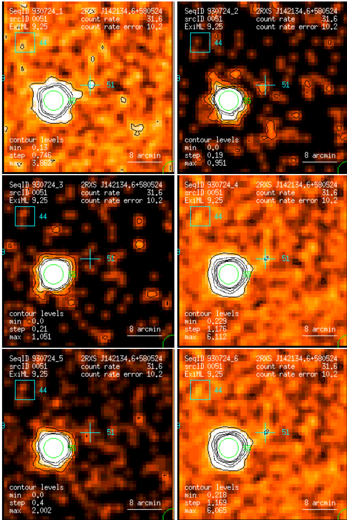
Figure 51: RASS 930724: detection 0051: band rate images, Gaussian filter: (1) PSPC channels 11 – 41, (2) 52 – 90, (3) 91 – 201, (4) 11 – 235, (5) 52 – 201, (6) 11 – 201. Broad band rates in counts/ks. Band rate contour levels in counts/ks/arcmin 2 .
