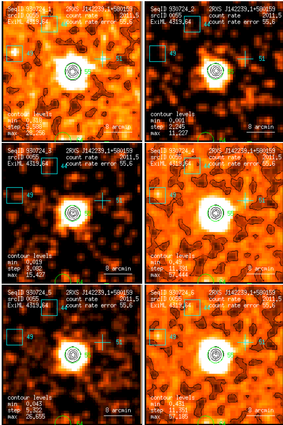
Figure 55: RASS 930724: detection 0055: band rate images, Gaussian filter: (1) PSPC channels 11 – 41, (2) 52 – 90, (3) 91 – 201, (4) 11 – 235, (5) 52 – 201, (6) 11 – 201. Broad band rates in counts/ks. Band rate contour levels in counts/ks/arcmin 2 .
