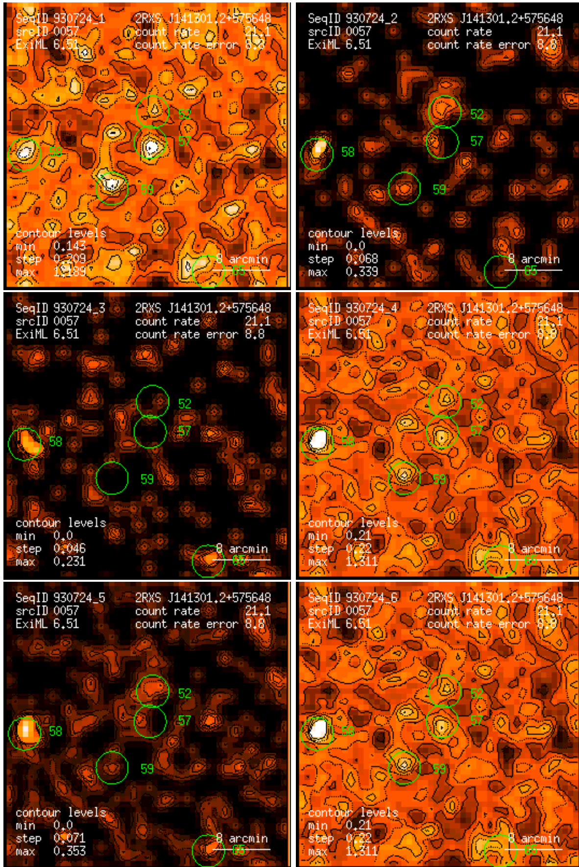
Figure 57: RASS 930724: detection 0057: band rate images, Gaussian filter: (1) PSPC channels 11 – 41, (2) 52 – 90, (3) 91 – 201, (4) 11 – 235, (5) 52 – 201, (6) 11 – 201. Broad band rates in counts/ks. Band rate contour levels in counts/ks/arcmin 2 .
