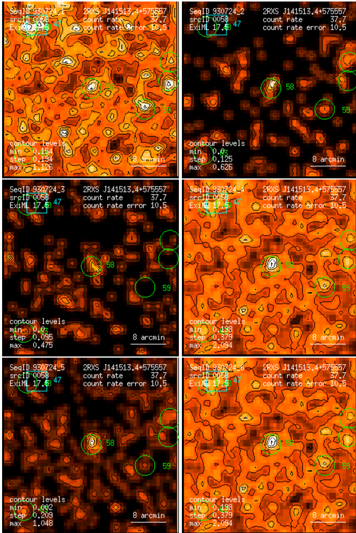
Figure 58: RASS 930724: detection 0058: band rate images, Gaussian filter: (1) PSPC channels 11 – 41, (2) 52 – 90, (3) 91 – 201, (4) 11 – 235, (5) 52 – 201, (6) 11 – 201. Broad band rates in counts/ks. Band rate contour levels in counts/ks/arcmin 2 .
