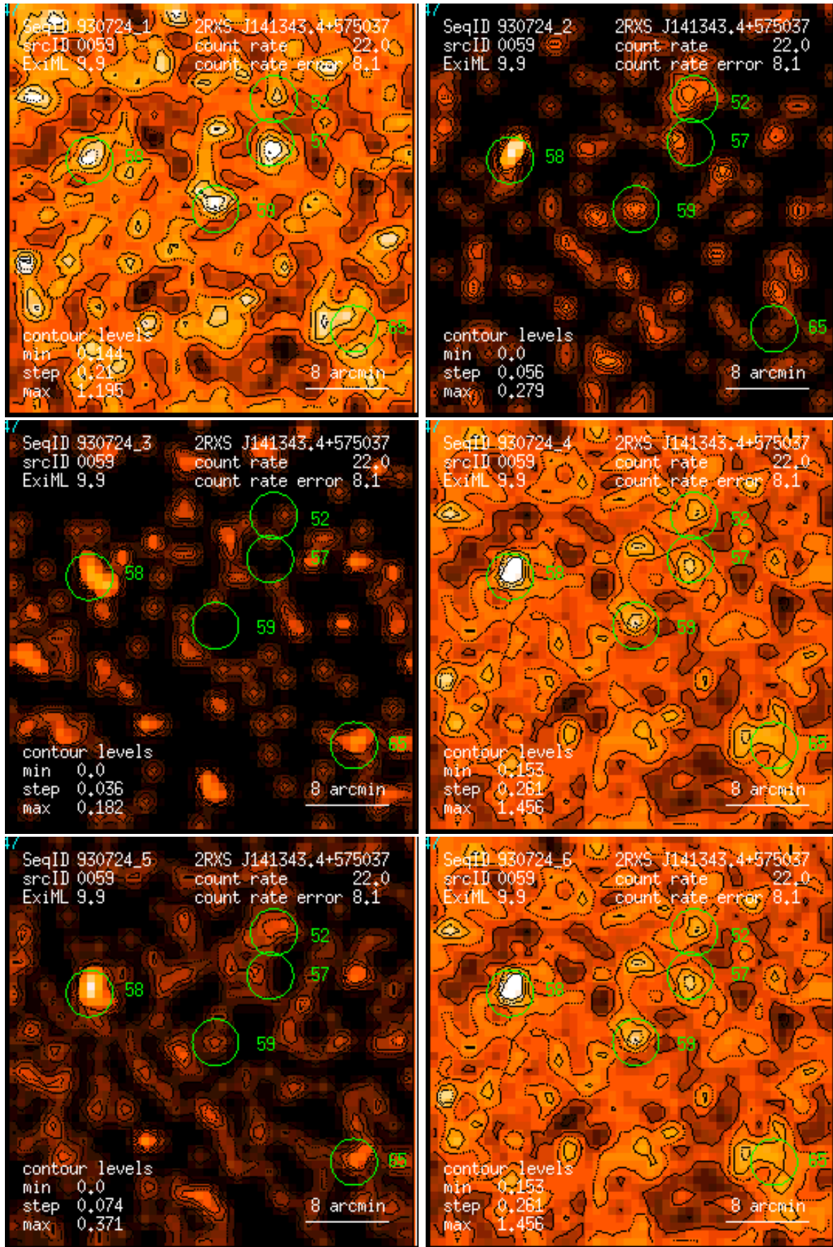
Figure 59: RASS 930724: detection 0059: band rate images, Gaussian filter: (1) PSPC channels 11 – 41, (2) 52 – 90, (3) 91 – 201, (4) 11 – 235, (5) 52 – 201, (6) 11 – 201. Broad band rates in counts/ks. Band rate contour levels in counts/ks/arcmin 2 .
