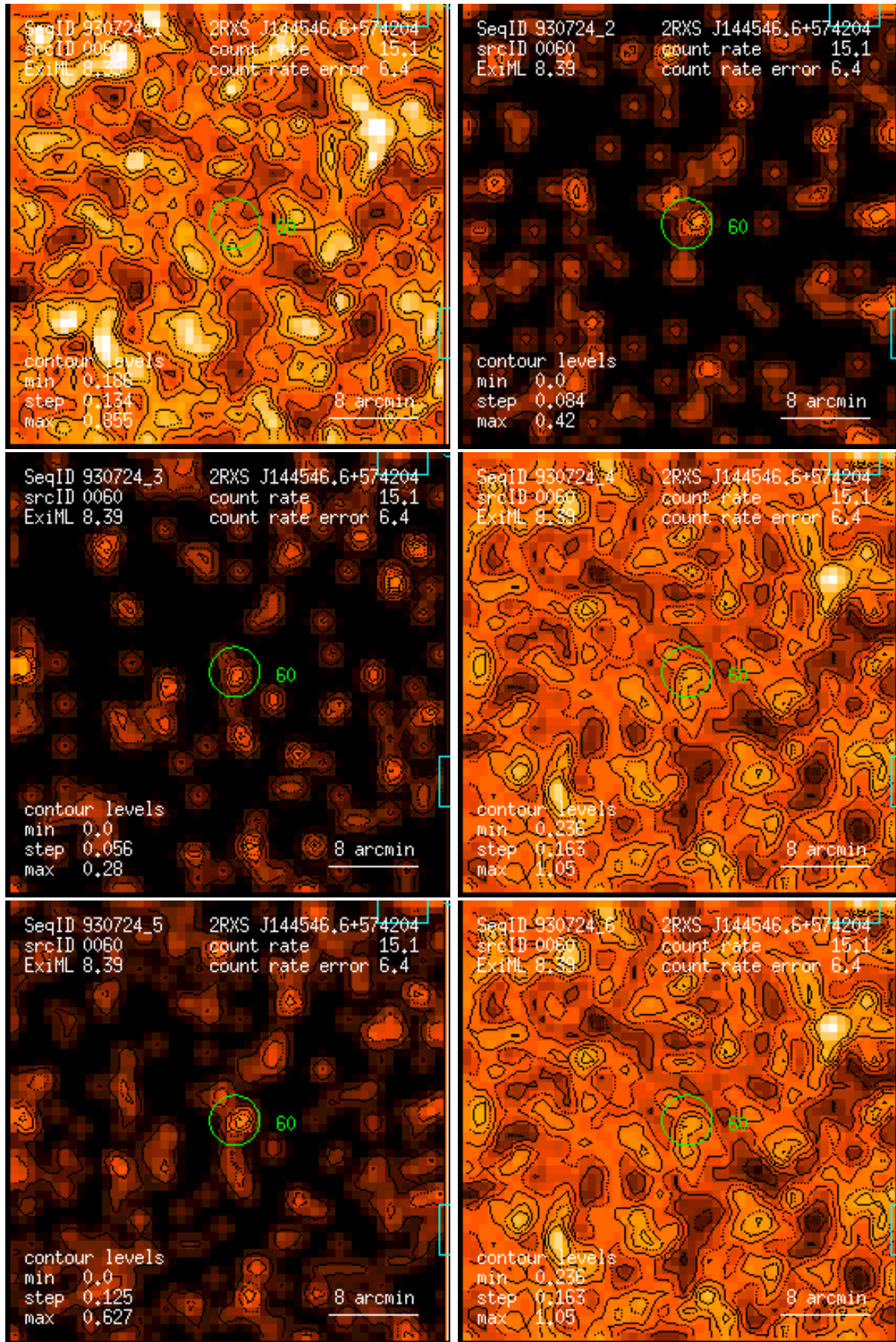
Figure 60: RASS 930724: detection 0060: band rate images, Gaussian filter: (1) PSPC channels 11 – 41, (2) 52 – 90, (3) 91 – 201, (4) 11 – 235, (5) 52 – 201, (6) 11 – 201. Broad band rates in counts/ks. Band rate contour levels in counts/ks/arcmin 2 .
