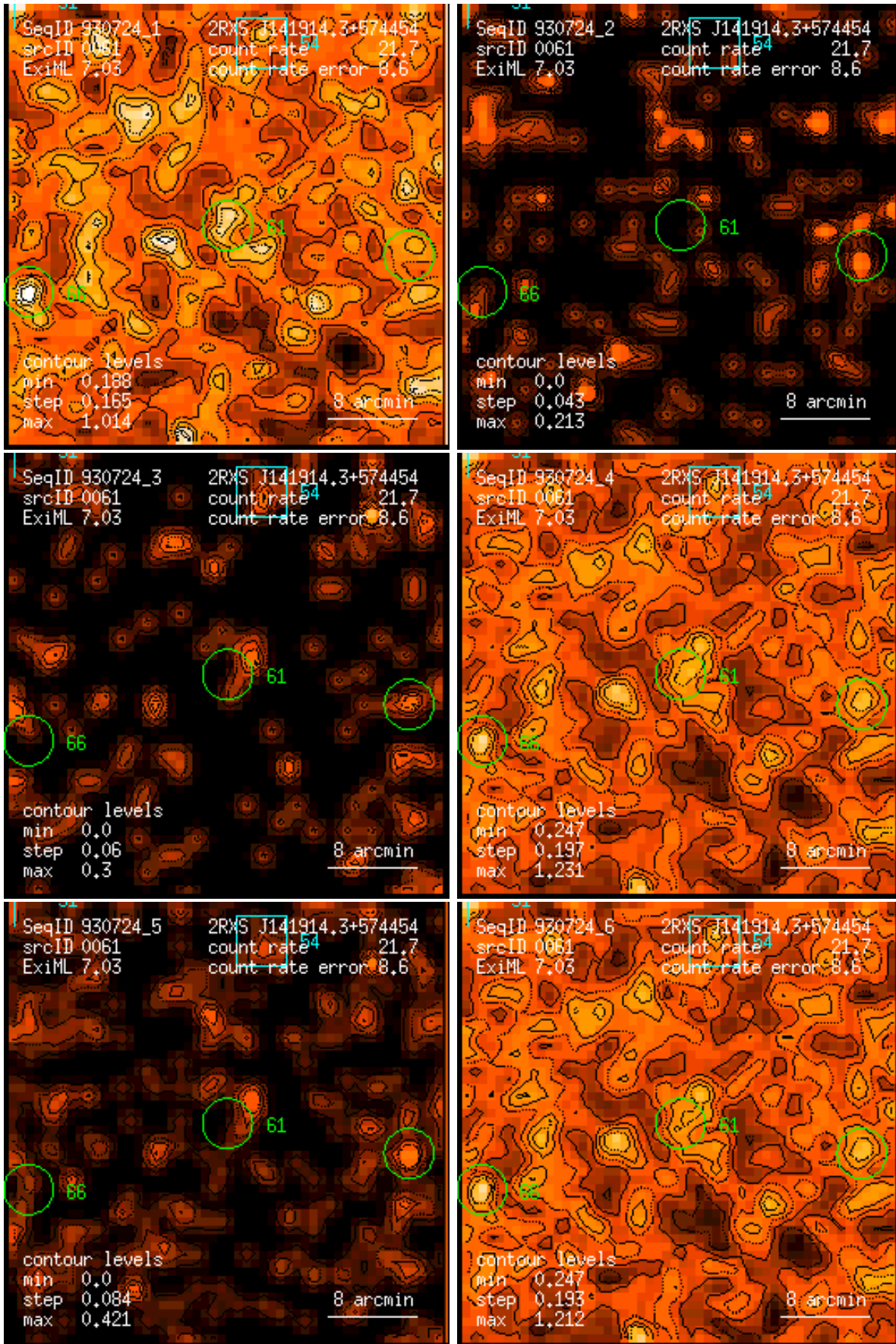
Figure 61: RASS 930724: detection 0061: band rate images, Gaussian filter: (1) PSPC channels 11 – 41, (2) 52 – 90, (3) 91 – 201, (4) 11 – 235, (5) 52 – 201, (6) 11 – 201. Broad band rates in counts/ks. Band rate contour levels in counts/ks/arcmin 2 .
