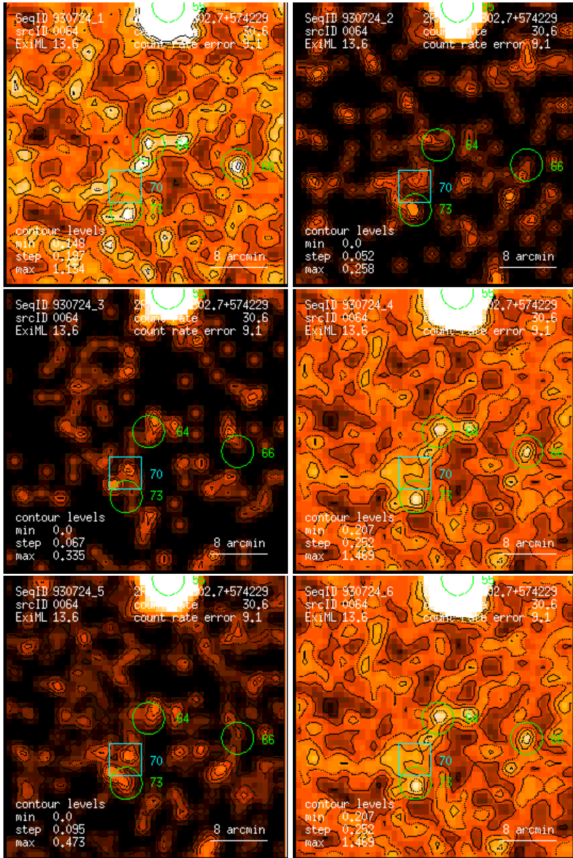
Figure 64: RASS 930724: detection 0064: band rate images, Gaussian filter: (1) PSPC channels 11 – 41, (2) 52 – 90, (3) 91 – 201, (4) 11 – 235, (5) 52 – 201, (6) 11 – 201. Broad band rates in counts/ks. Band rate contour levels in counts/ks/arcmin 2 .
