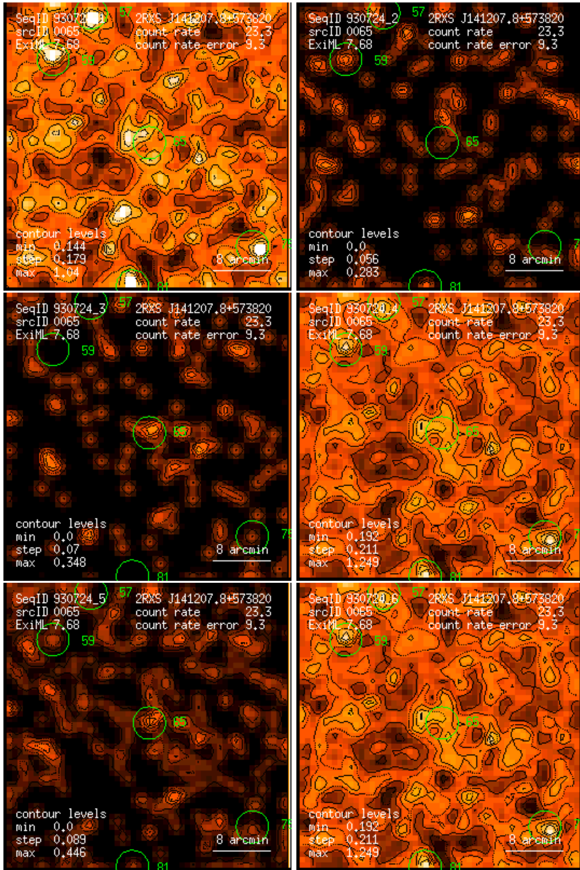
Figure 65: RASS 930724: detection 0065: band rate images, Gaussian filter: (1) PSPC channels 11 – 41, (2) 52 – 90, (3) 91 – 201, (4) 11 – 235, (5) 52 – 201, (6) 11 – 201. Broad band rates in counts/ks. Band rate contour levels in counts/ks/arcmin 2 .
