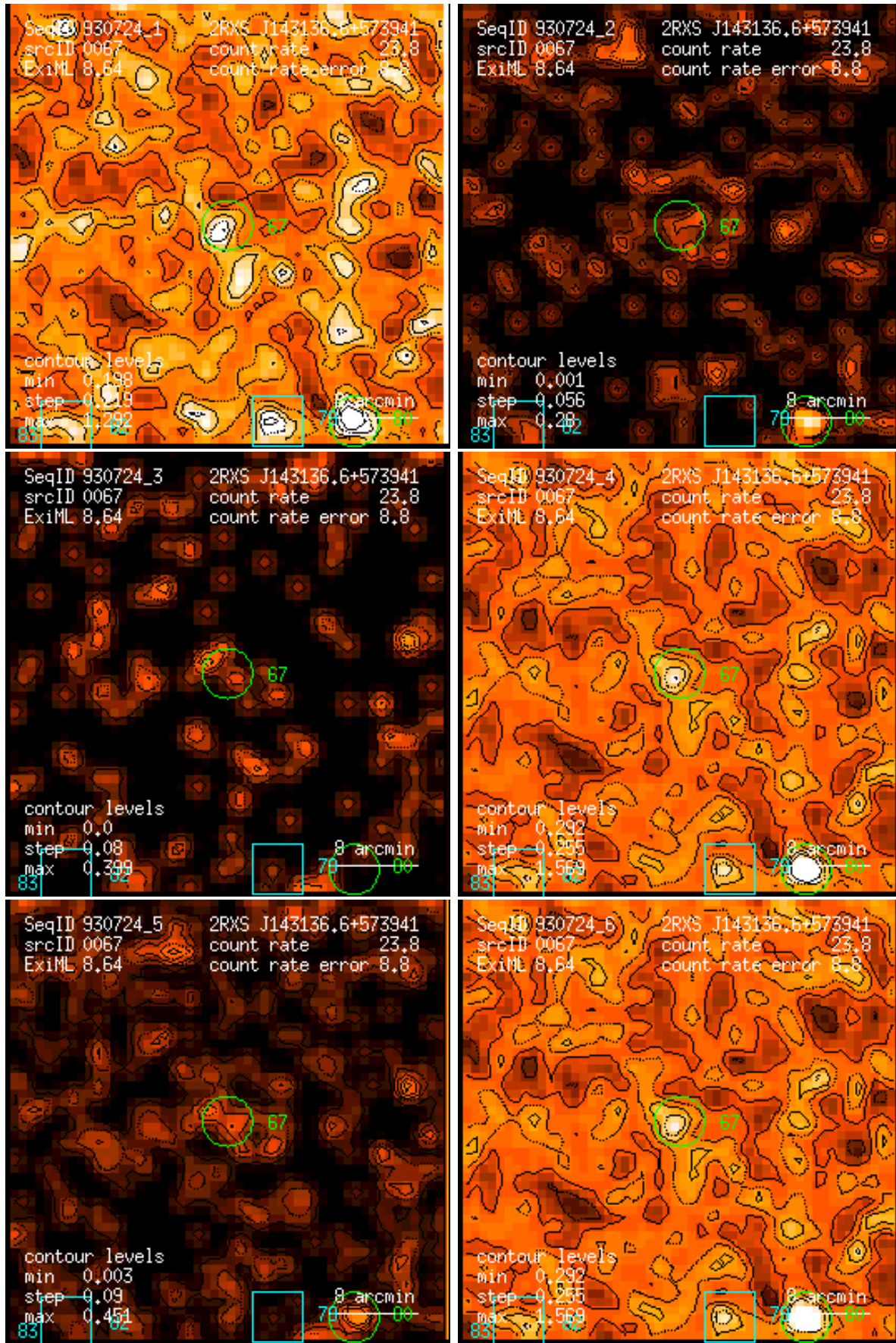
Figure 67: RASS 930724: detection 0067: band rate images, Gaussian filter: (1) PSPC channels 11 – 41, (2) 52 – 90, (3) 91 – 201, (4) 11 – 235, (5) 52 – 201, (6) 11 – 201. Broad band rates in counts/ks. Band rate contour levels in counts/ks/arcmin 2 .
