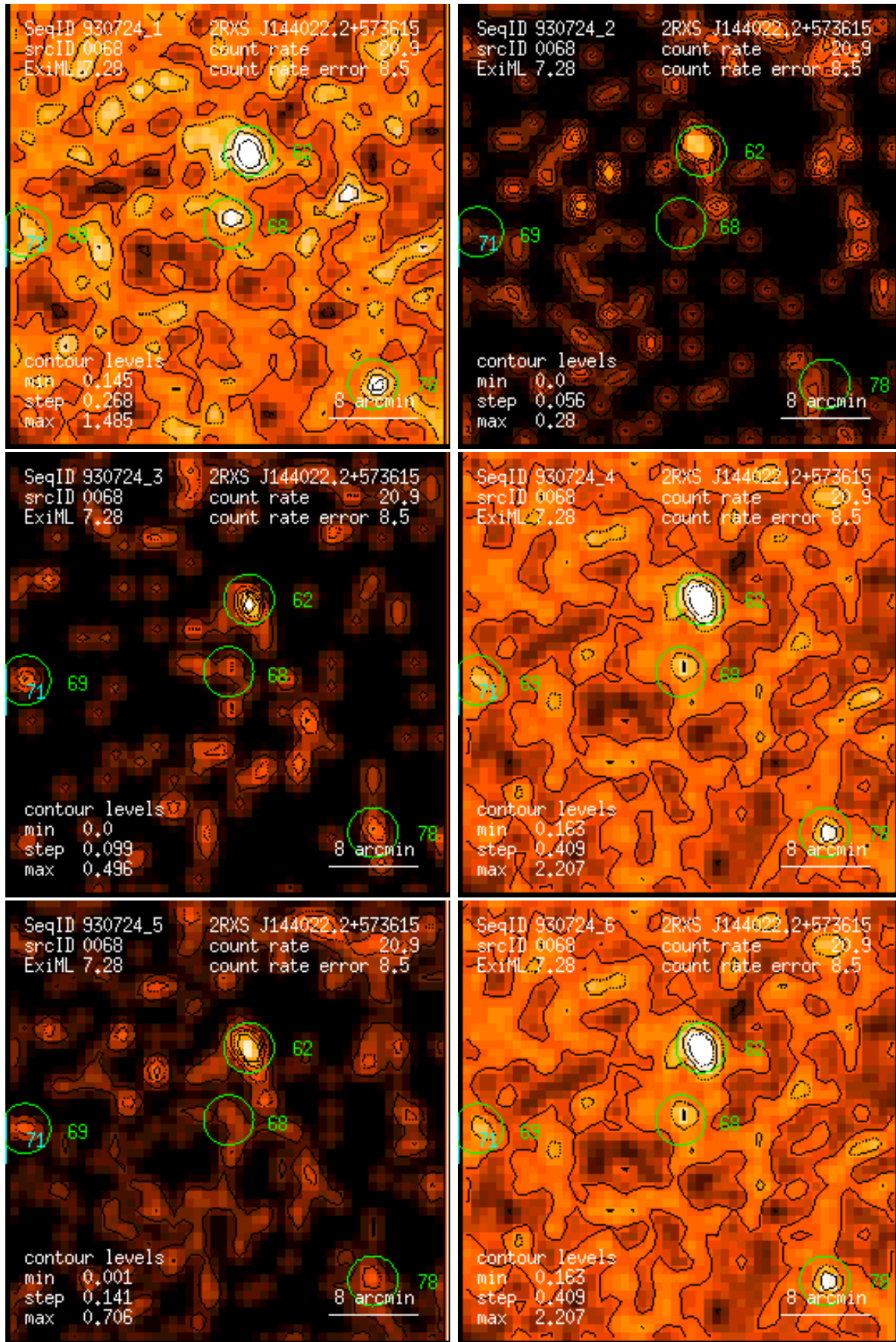
Figure 68: RASS 930724: detection 0068: band rate images, Gaussian filter: (1) PSPC channels 11 – 41, (2) 52 – 90, (3) 91 – 201, (4) 11 – 235, (5) 52 – 201, (6) 11 – 201. Broad band rates in counts/ks. Band rate contour levels in counts/ks/arcmin 2 .
