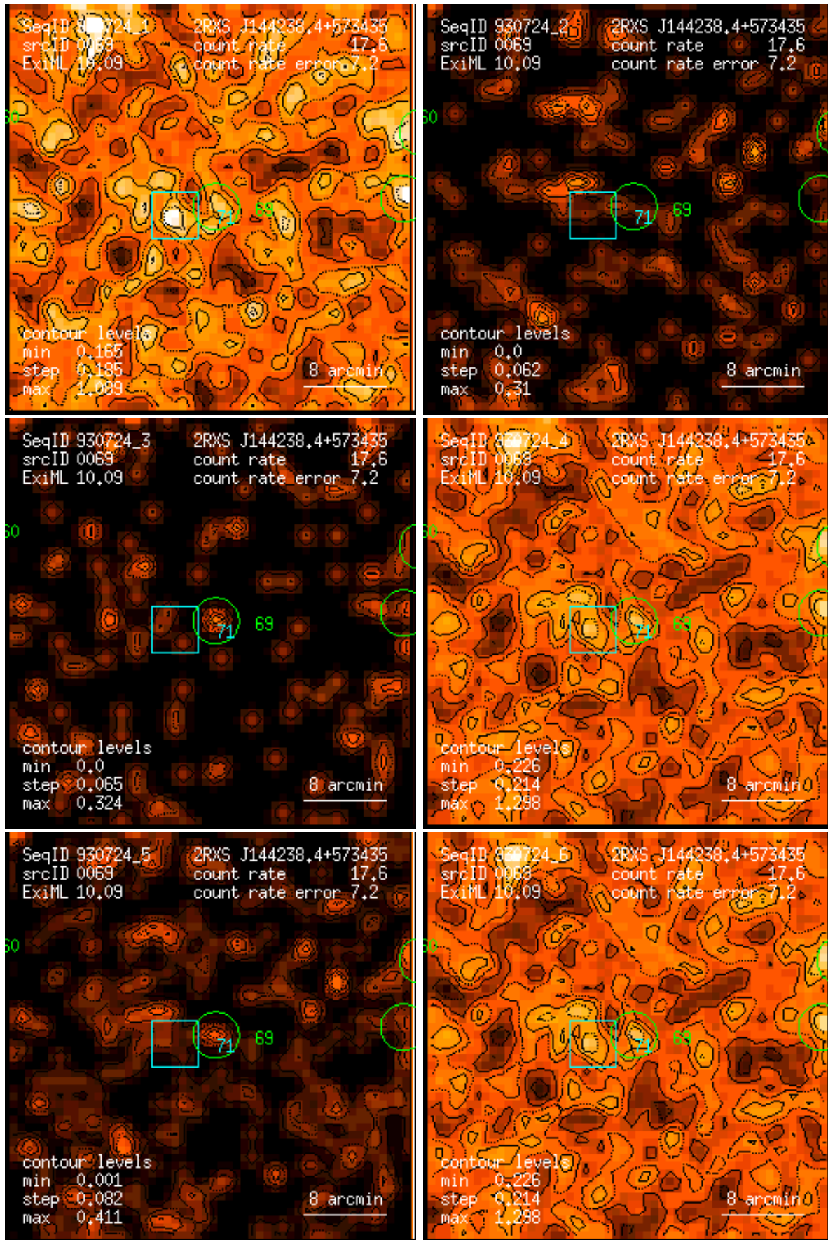
Figure 69: RASS 930724: detection 0069: band rate images, Gaussian filter: (1) PSPC channels 11 – 41, (2) 52 – 90, (3) 91 – 201, (4) 11 – 235, (5) 52 – 201, (6) 11 – 201. Broad band rates in counts/ks. Band rate contour levels in counts/ks/arcmin 2 .
