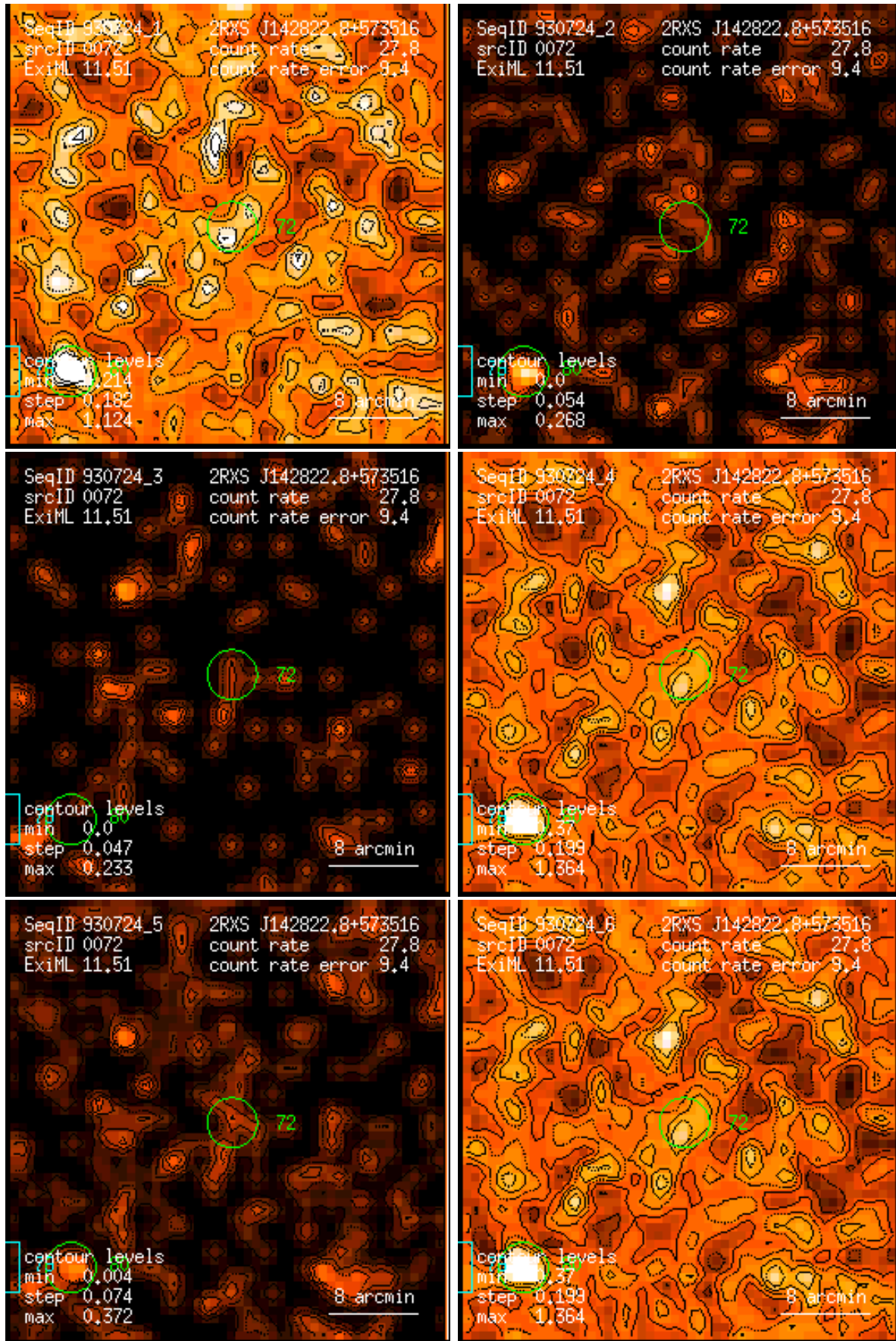
Figure 72: RASS 930724: detection 0072: band rate images, Gaussian filter: (1) PSPC channels 11 – 41, (2) 52 – 90, (3) 91 – 201, (4) 11 – 235, (5) 52 – 201, (6) 11 – 201. Broad band rates in counts/ks. Band rate contour levels in counts/ks/arcmin 2 .
