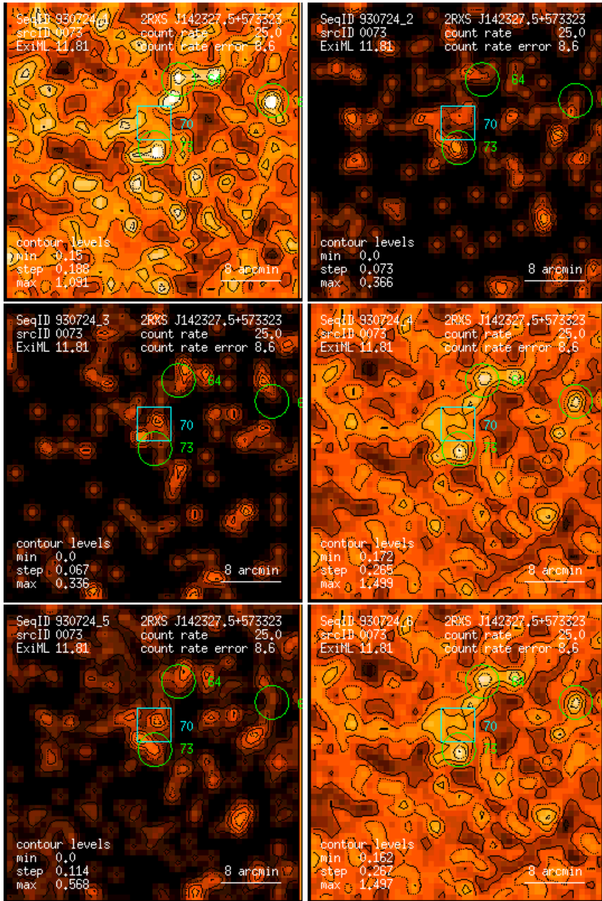
Figure 73: RASS 930724: detection 0073: band rate images, Gaussian filter: (1) PSPC channels 11 – 41, (2) 52 – 90, (3) 91 – 201, (4) 11 – 235, (5) 52 – 201, (6) 11 – 201. Broad band rates in counts/ks. Band rate contour levels in counts/ks/arcmin 2 .
