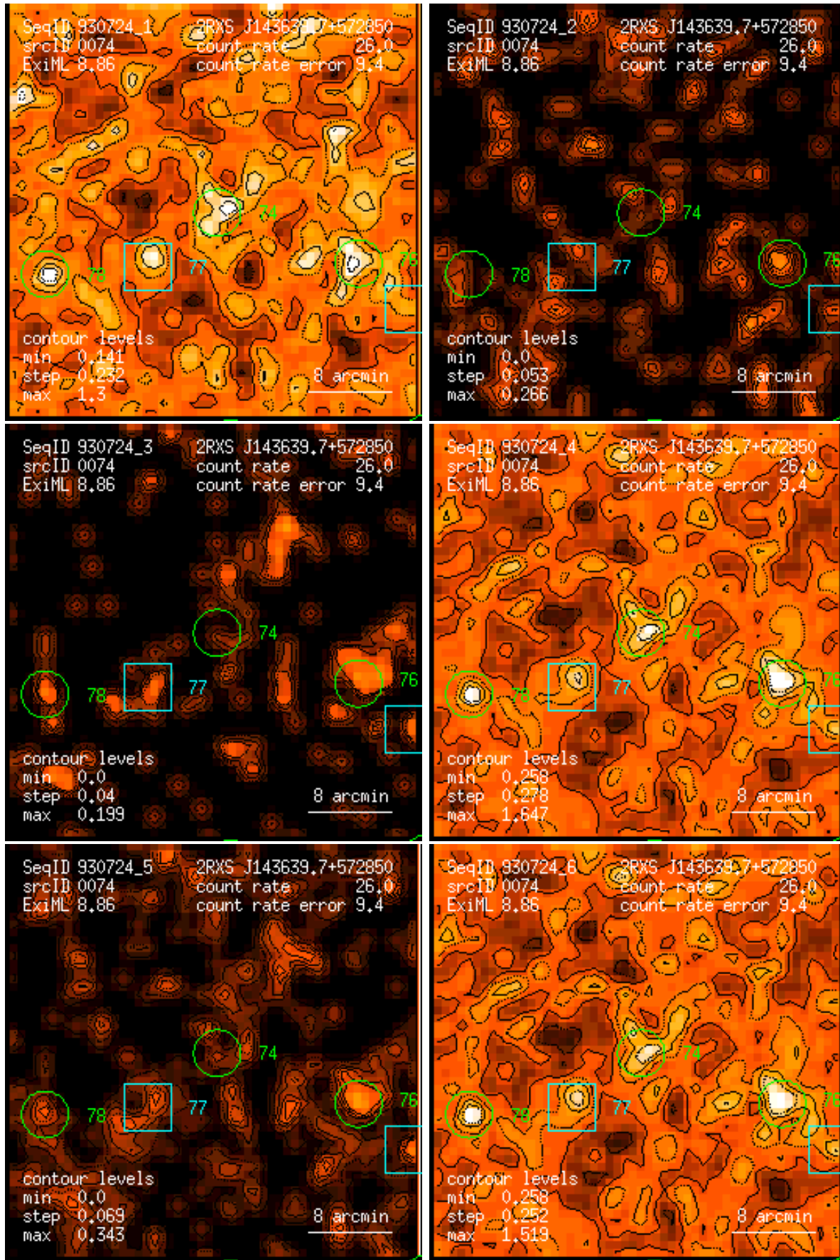
Figure 74: RASS 930724: detection 0074: band rate images, Gaussian filter: (1) PSPC channels 11 – 41, (2) 52 – 90, (3) 91 – 201, (4) 11 – 235, (5) 52 – 201, (6) 11 – 201. Broad band rates in counts/ks. Band rate contour levels in counts/ks/arcmin 2 .
