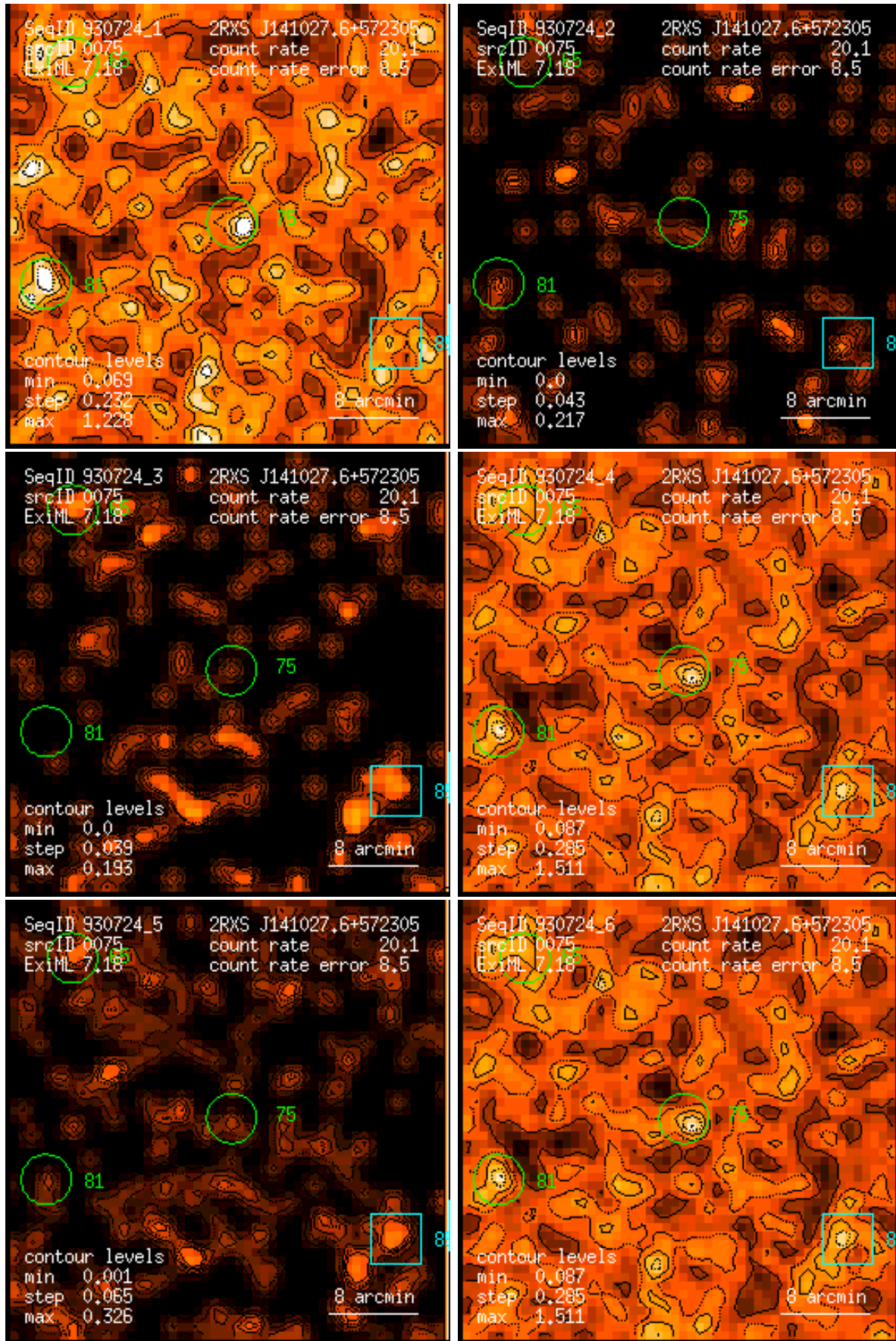
Figure 75: RASS 930724: detection 0075: band rate images, Gaussian filter: (1) PSPC channels 11 – 41, (2) 52 – 90, (3) 91 – 201, (4) 11 – 235, (5) 52 – 201, (6) 11 – 201. Broad band rates in counts/ks. Band rate contour levels in counts/ks/arcmin 2 .
