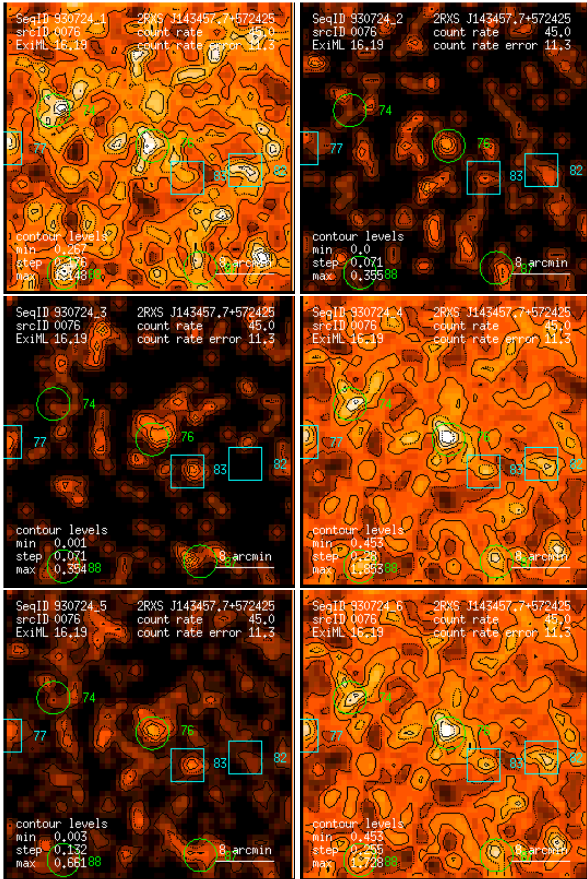
Figure 76: RASS 930724: detection 0076: band rate images, Gaussian filter: (1) PSPC channels 11 – 41, (2) 52 – 90, (3) 91 – 201, (4) 11 – 235, (5) 52 – 201, (6) 11 – 201. Broad band rates in counts/ks. Band rate contour levels in counts/ks/arcmin 2 .
