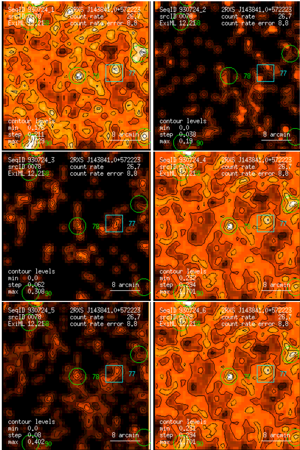
Figure 78: RASS 930724: detection 0078: band rate images, Gaussian filter: (1) PSPC channels 11 – 41, (2) 52 – 90, (3) 91 – 201, (4) 11 – 235, (5) 52 – 201, (6) 11 – 201. Broad band rates in counts/ks. Band rate contour levels in counts/ks/arcmin 2 .
