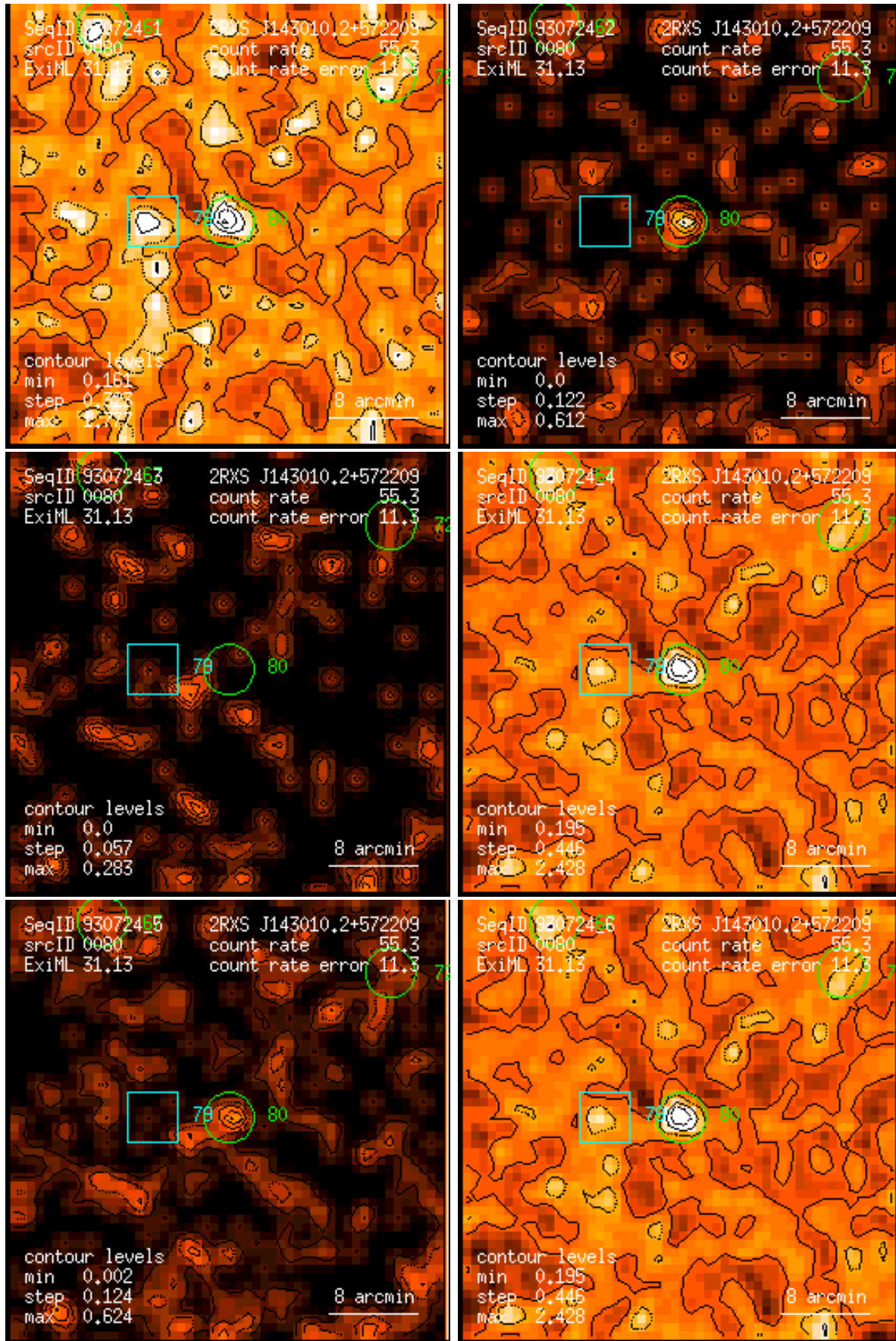
Figure 80: RASS 930724: detection 0080: band rate images, Gaussian filter: (1) PSPC channels 11 – 41, (2) 52 – 90, (3) 91 – 201, (4) 11 – 235, (5) 52 – 201, (6) 11 – 201. Broad band rates in counts/ks. Band rate contour levels in counts/ks/arcmin 2 .
