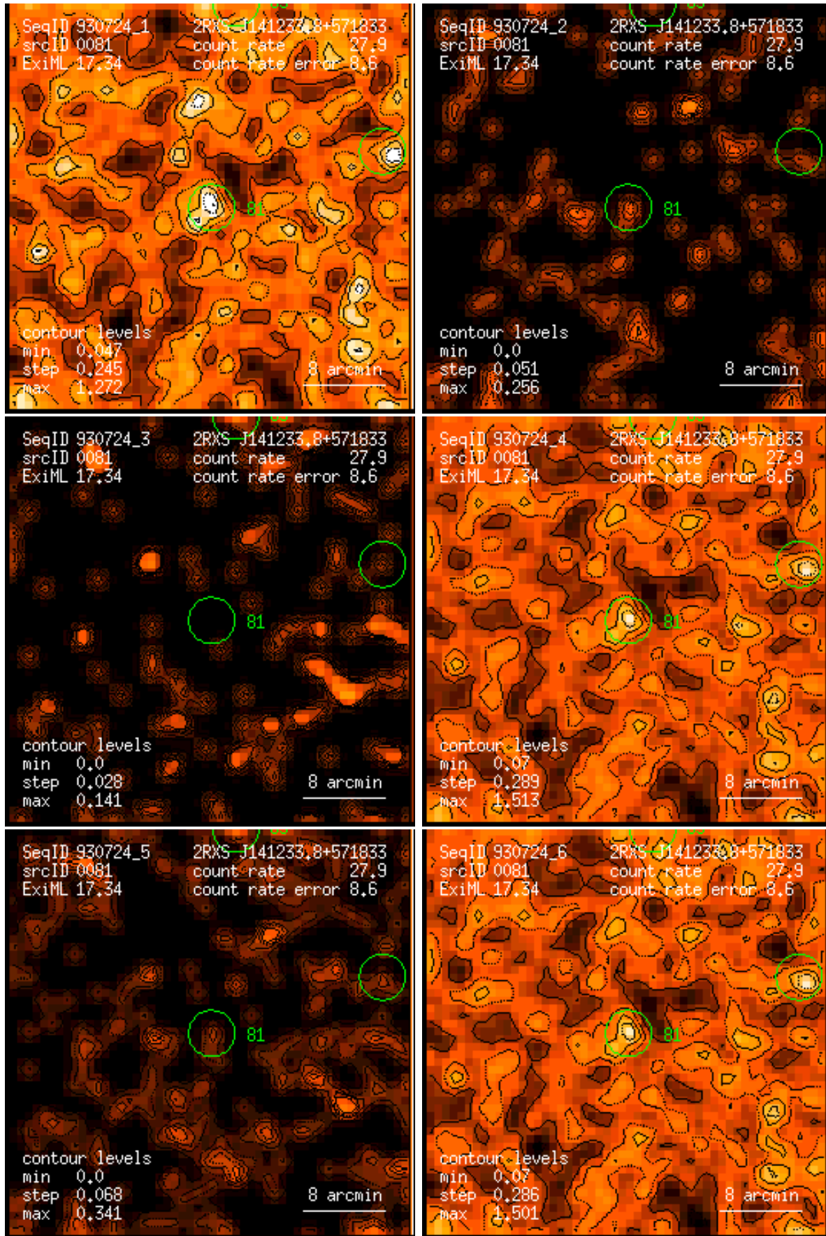
Figure 81: RASS 930724: detection 0081: band rate images, Gaussian filter: (1) PSPC channels 11 – 41, (2) 52 – 90, (3) 91 – 201, (4) 11 – 235, (5) 52 – 201, (6) 11 – 201. Broad band rates in counts/ks. Band rate contour levels in counts/ks/arcmin 2 .
