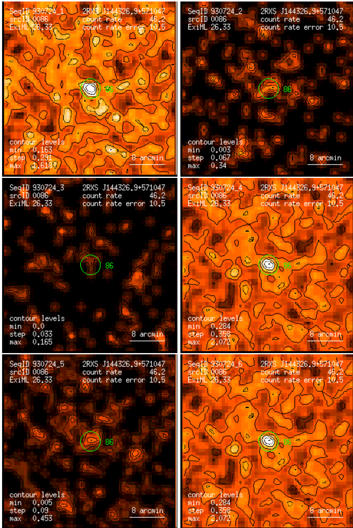
Figure 86: RASS 930724: detection 0086: band rate images, Gaussian filter: (1) PSPC channels 11 – 41, (2) 52 – 90, (3) 91 – 201, (4) 11 – 235, (5) 52 – 201, (6) 11 – 201. Broad band rates in counts/ks. Band rate contour levels in counts/ks/arcmin 2 .
