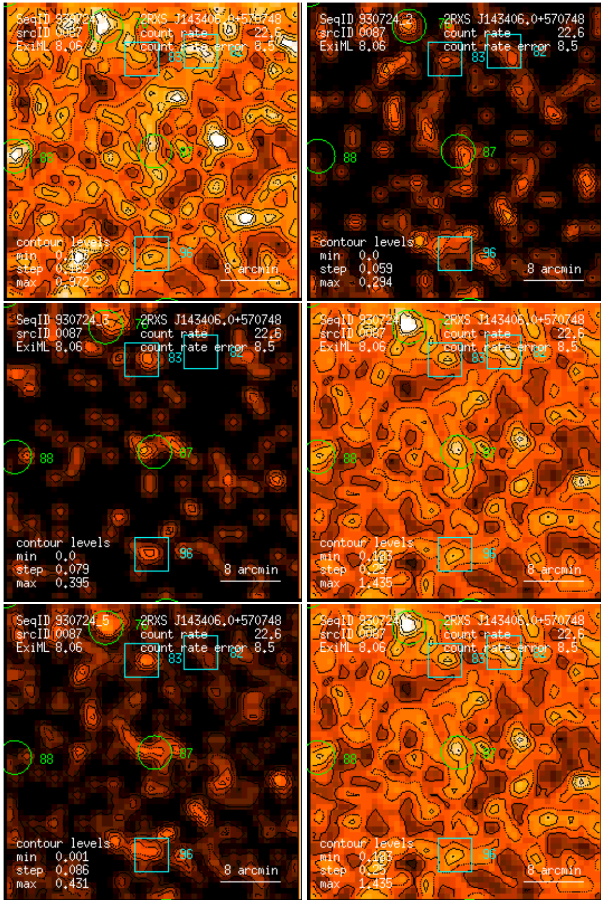
Figure 87: RASS 930724: detection 0087: band rate images, Gaussian filter: (1) PSPC channels 11 – 41, (2) 52 – 90, (3) 91 – 201, (4) 11 – 235, (5) 52 – 201, (6) 11 – 201. Broad band rates in counts/ks. Band rate contour levels in counts/ks/arcmin 2 .
