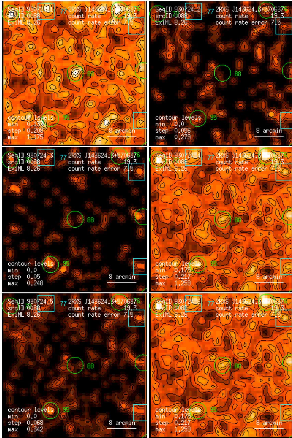
Figure 88: RASS 930724: detection 0088: band rate images, Gaussian filter: (1) PSPC channels 11 – 41, (2) 52 – 90, (3) 91 – 201, (4) 11 – 235, (5) 52 – 201, (6) 11 – 201. Broad band rates in counts/ks. Band rate contour levels in counts/ks/arcmin 2 .
