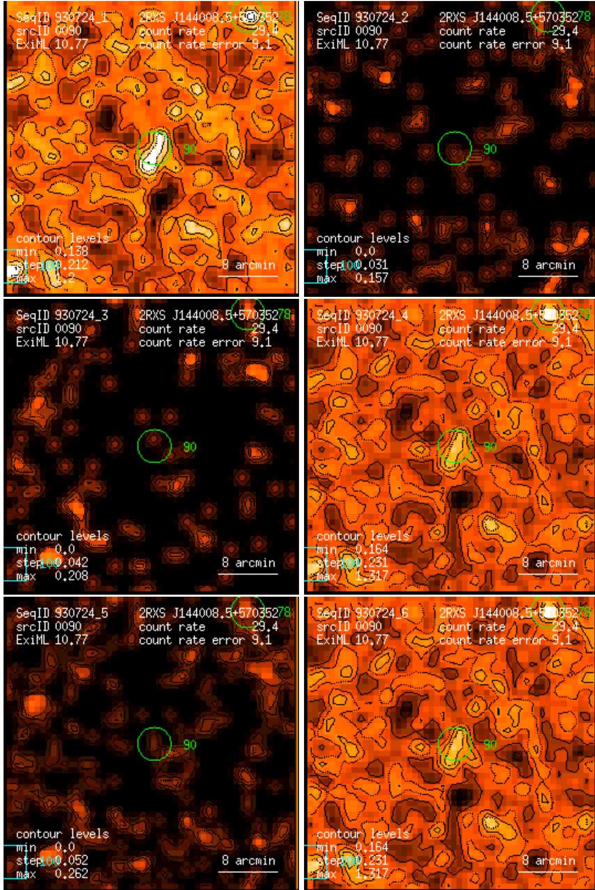
Figure 90: RASS 930724: detection 0090: band rate images, Gaussian filter: (1) PSPC channels 11 – 41, (2) 52 – 90, (3) 91 – 201, (4) 11 – 235, (5) 52 – 201, (6) 11 – 201. Broad band rates in counts/ks. Band rate contour levels in counts/ks/arcmin 2 .
