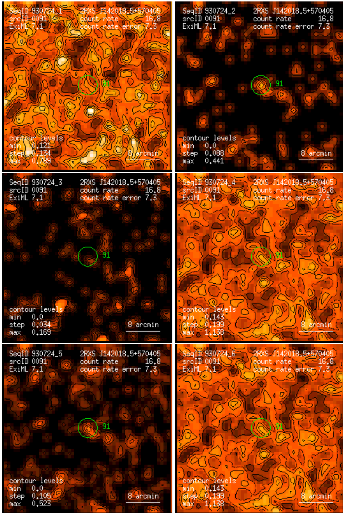
Figure 91: RASS 930724: detection 0091: band rate images, Gaussian filter: (1) PSPC channels 11 – 41, (2) 52 – 90, (3) 91 – 201, (4) 11 – 235, (5) 52 – 201, (6) 11 – 201. Broad band rates in counts/ks. Band rate contour levels in counts/ks/arcmin 2 .
