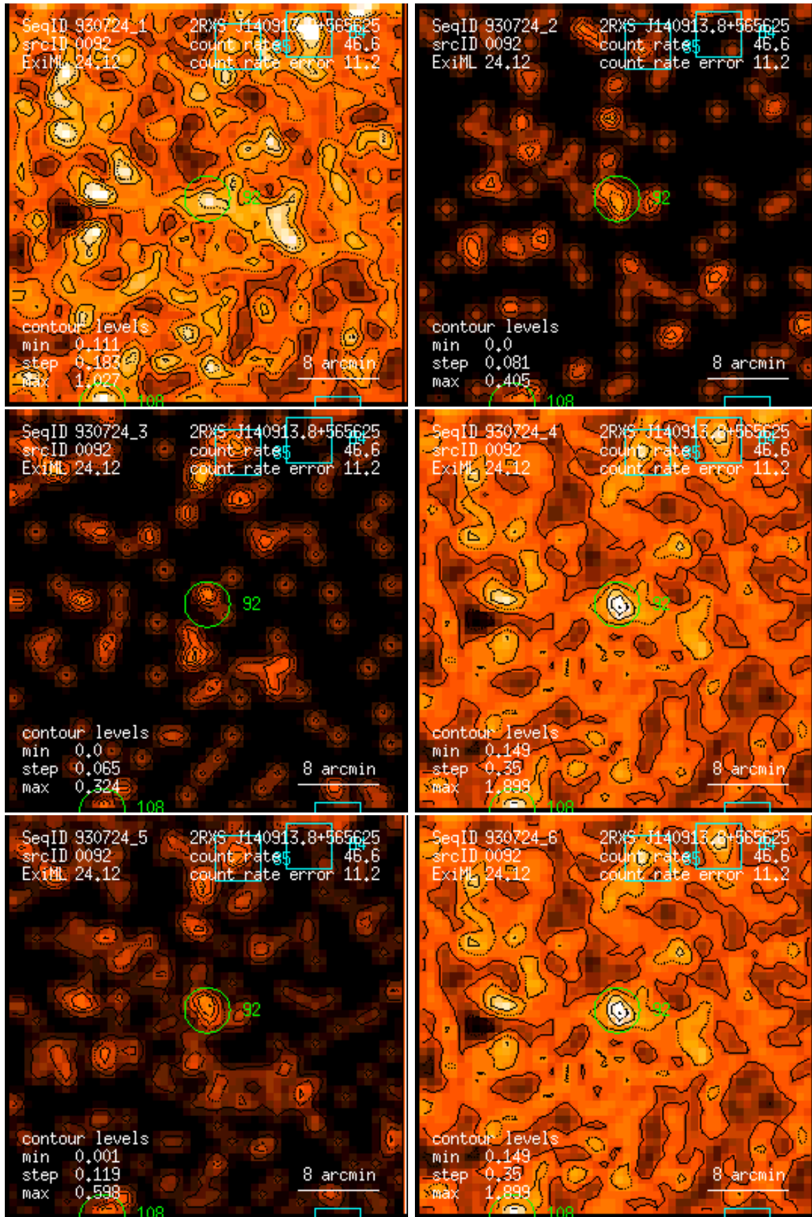
Figure 92: RASS 930724: detection 0092: band rate images, Gaussian filter: (1) PSPC channels 11 – 41, (2) 52 – 90, (3) 91 – 201, (4) 11 – 235, (5) 52 – 201, (6) 11 – 201. Broad band rates in counts/ks. Band rate contour levels in counts/ks/arcmin 2 .
