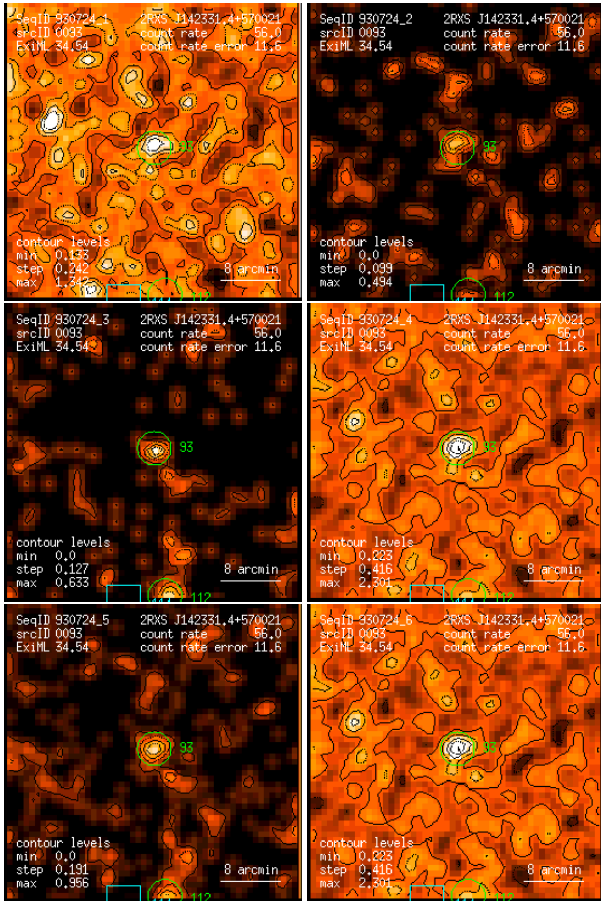
Figure 93: RASS 930724: detection 0093: band rate images, Gaussian filter: (1) PSPC channels 11 – 41, (2) 52 – 90, (3) 91 – 201, (4) 11 – 235, (5) 52 – 201, (6) 11 – 201. Broad band rates in counts/ks. Band rate contour levels in counts/ks/arcmin 2 .
