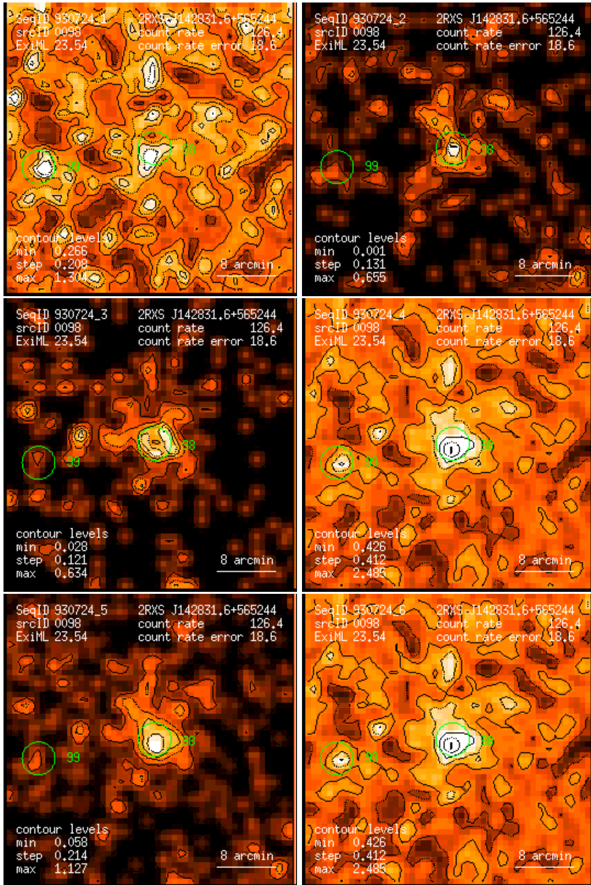
Figure 98: RASS 930724: detection 0098: band rate images, Gaussian filter: (1) PSPC channels 11 – 41, (2) 52 – 90, (3) 91 – 201, (4) 11 – 235, (5) 52 – 201, (6) 11 – 201. Broad band rates in counts/ks. Band rate contour levels in counts/ks/arcmin 2 .
