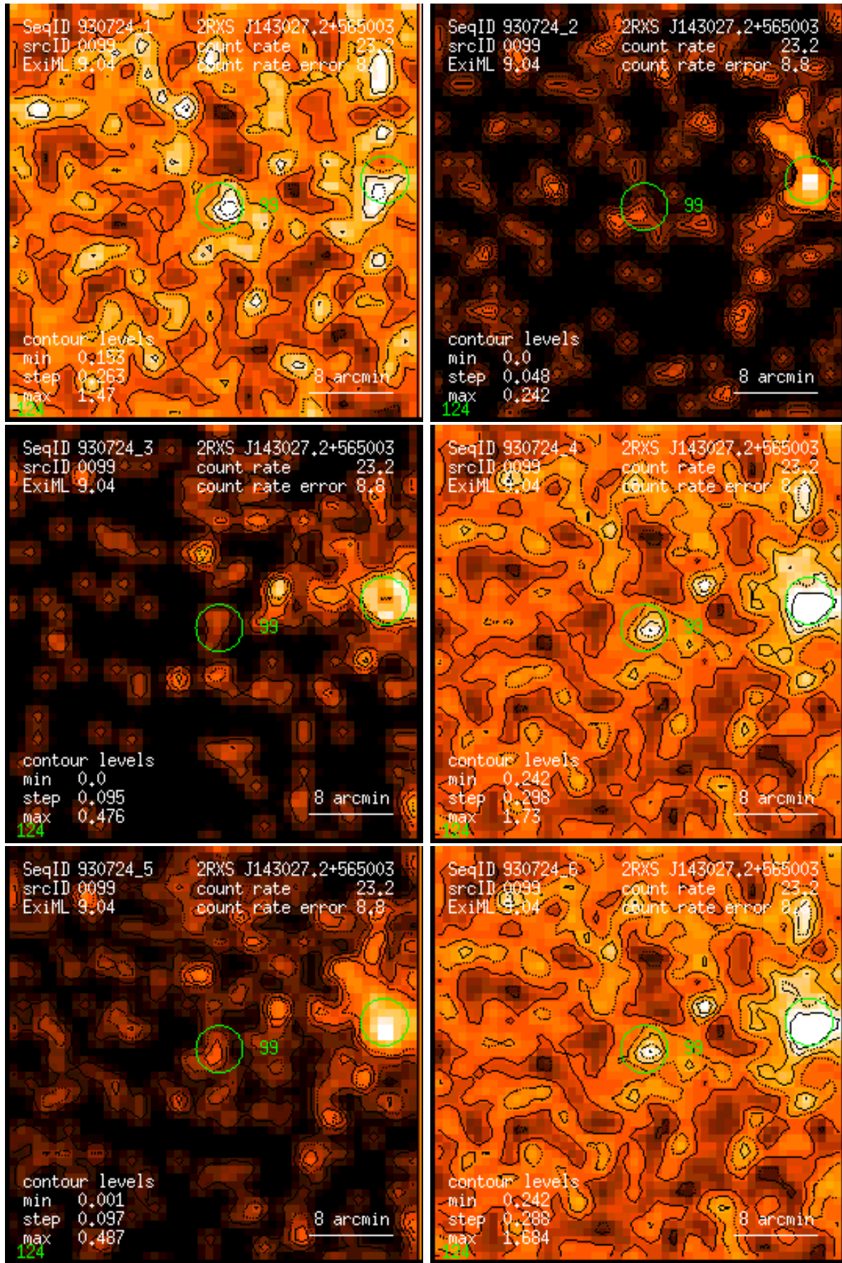
Figure 99: RASS 930724: detection 0099: band rate images, Gaussian filter: (1) PSPC channels 11 – 41, (2) 52 – 90, (3) 91 – 201, (4) 11 – 235, (5) 52 – 201, (6) 11 – 201. Broad band rates in counts/ks. Band rate contour levels in counts/ks/arcmin 2 .
