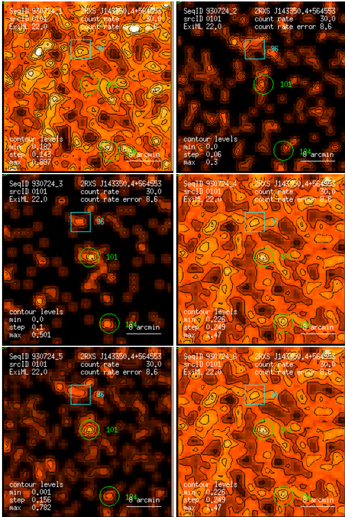
Figure 101: RASS 930724: detection 0101: band rate images, Gaussian filter: (1) PSPC channels 11 – 41, (2) 52 – 90, (3) 91 – 201, (4) 11 – 235, (5) 52 – 201, (6) 11 – 201. Broad band rates in counts/ks. Band rate contour levels in counts/ks/arcmin 2 .
