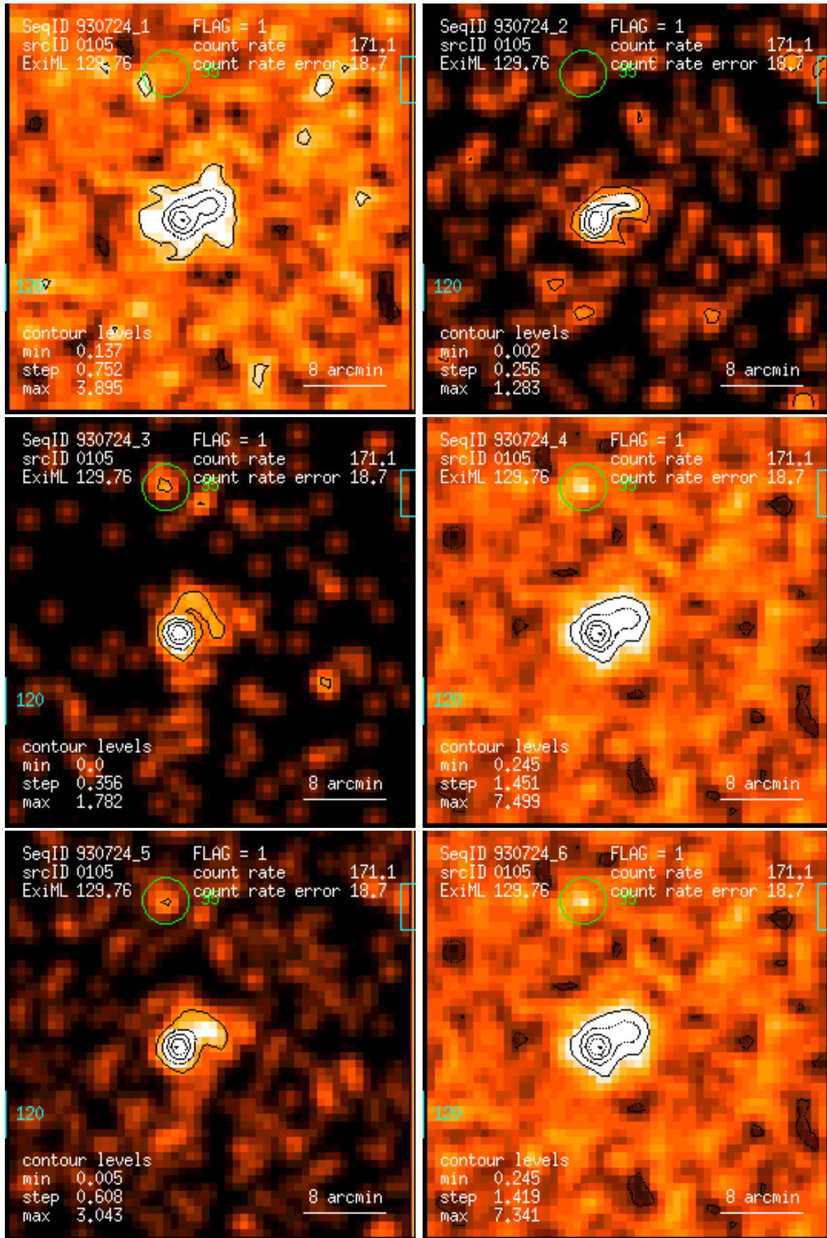
Figure 105: RASS 930724: detection 0105: band rate images, Gaussian filter: (1) PSPC channels 11 – 41, (2) 52 – 90, (3) 91 – 201, (4) 11 – 235, (5) 52 – 201, (6) 11 – 201. Broad band rates in counts/ks. Band rate contour levels in counts/ks/arcmin 2 .
