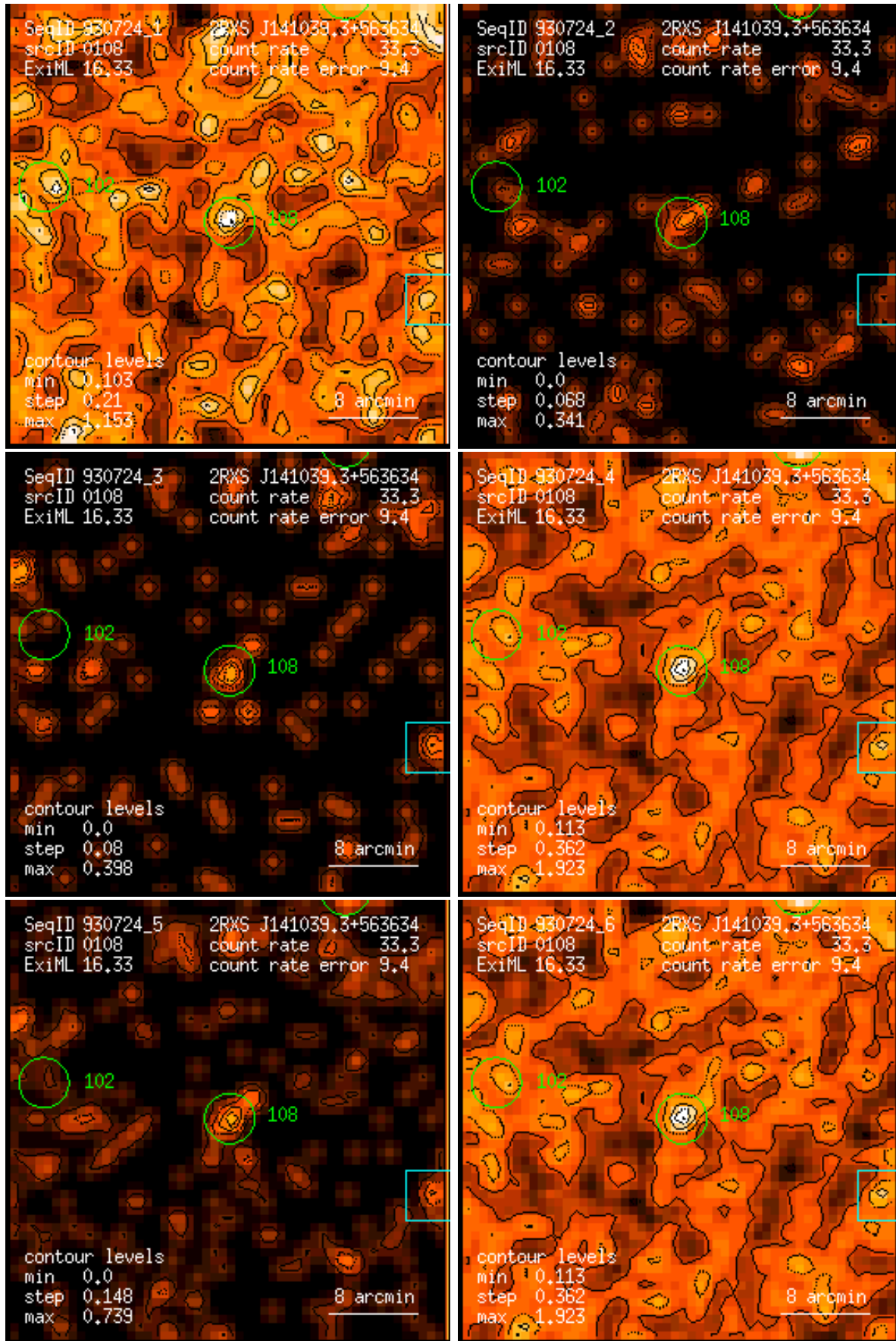
Figure 108: RASS 930724: detection 0108: band rate images, Gaussian filter: (1) PSPC channels 11 – 41, (2) 52 – 90, (3) 91 – 201, (4) 11 – 235, (5) 52 – 201, (6) 11 – 201. Broad band rates in counts/ks. Band rate contour levels in counts/ks/arcmin 2 .
