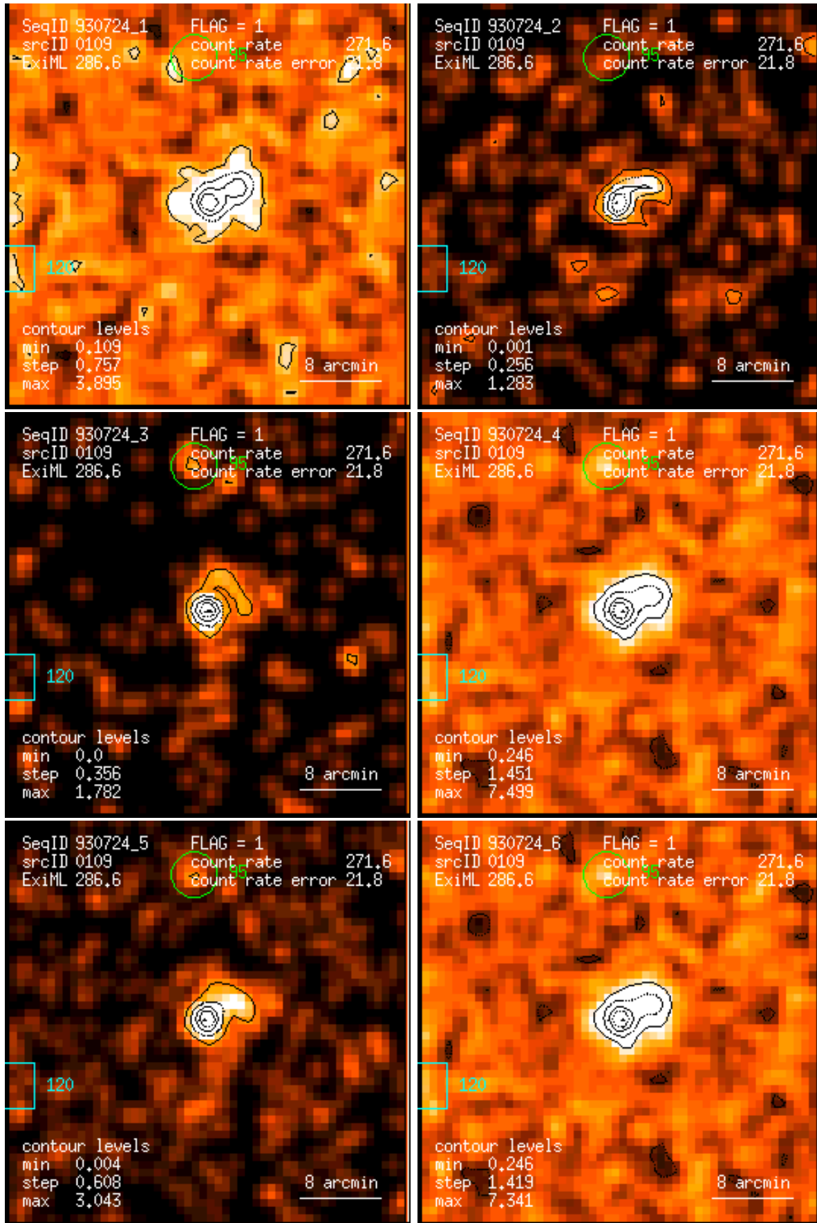
Figure 109: RASS 930724: detection 0109: band rate images, Gaussian filter: (1) PSPC channels 11 – 41, (2) 52 – 90, (3) 91 – 201, (4) 11 – 235, (5) 52 – 201, (6) 11 – 201. Broad band rates in counts/ks. Band rate contour levels in counts/ks/arcmin 2 .
