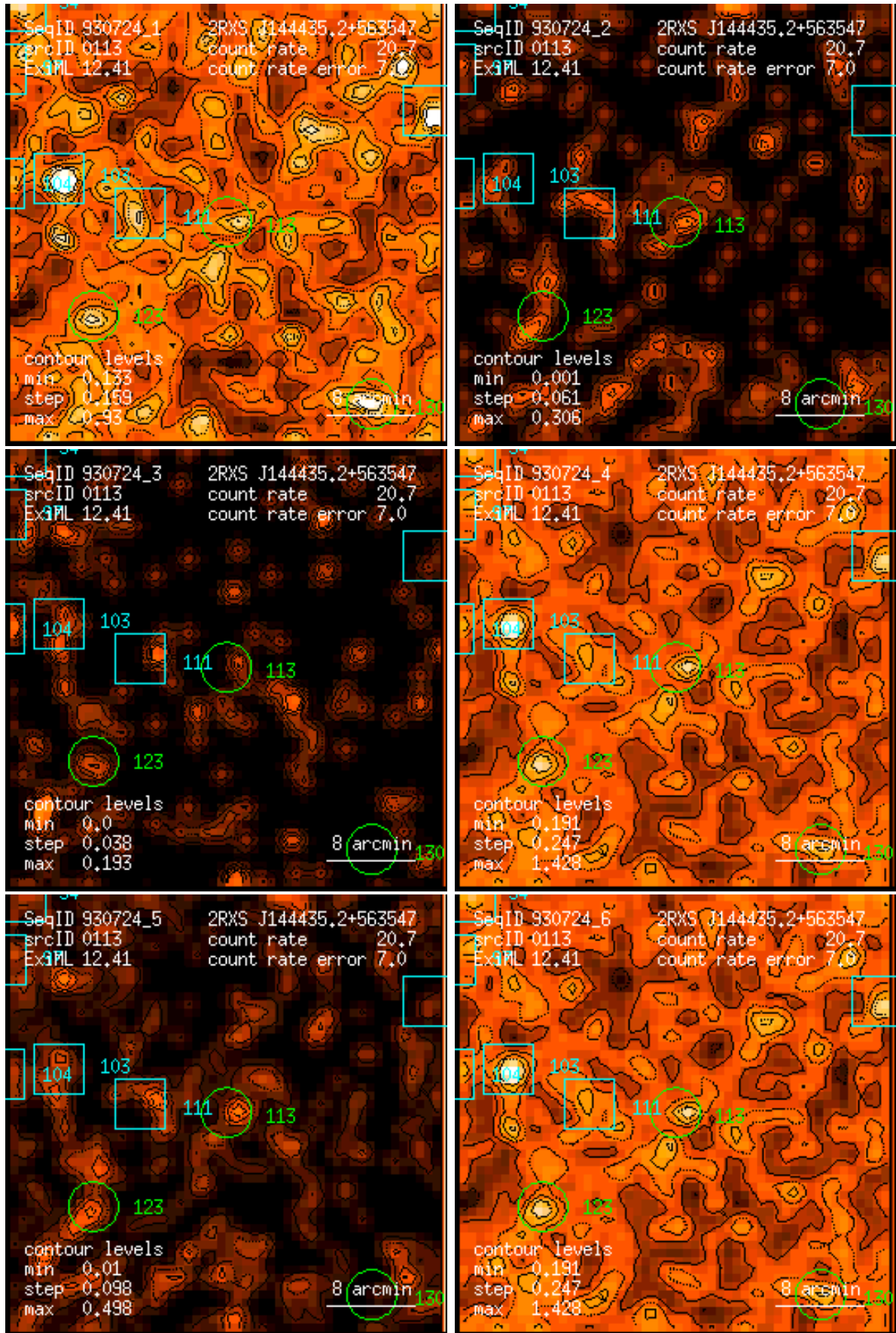
Figure 113: RASS 930724: detection 0113: band rate images, Gaussian filter: (1) PSPC channels 11 – 41, (2) 52 – 90, (3) 91 – 201, (4) 11 – 235, (5) 52 – 201, (6) 11 – 201. Broad band rates in counts/ks. Band rate contour levels in counts/ks/arcmin 2 .
