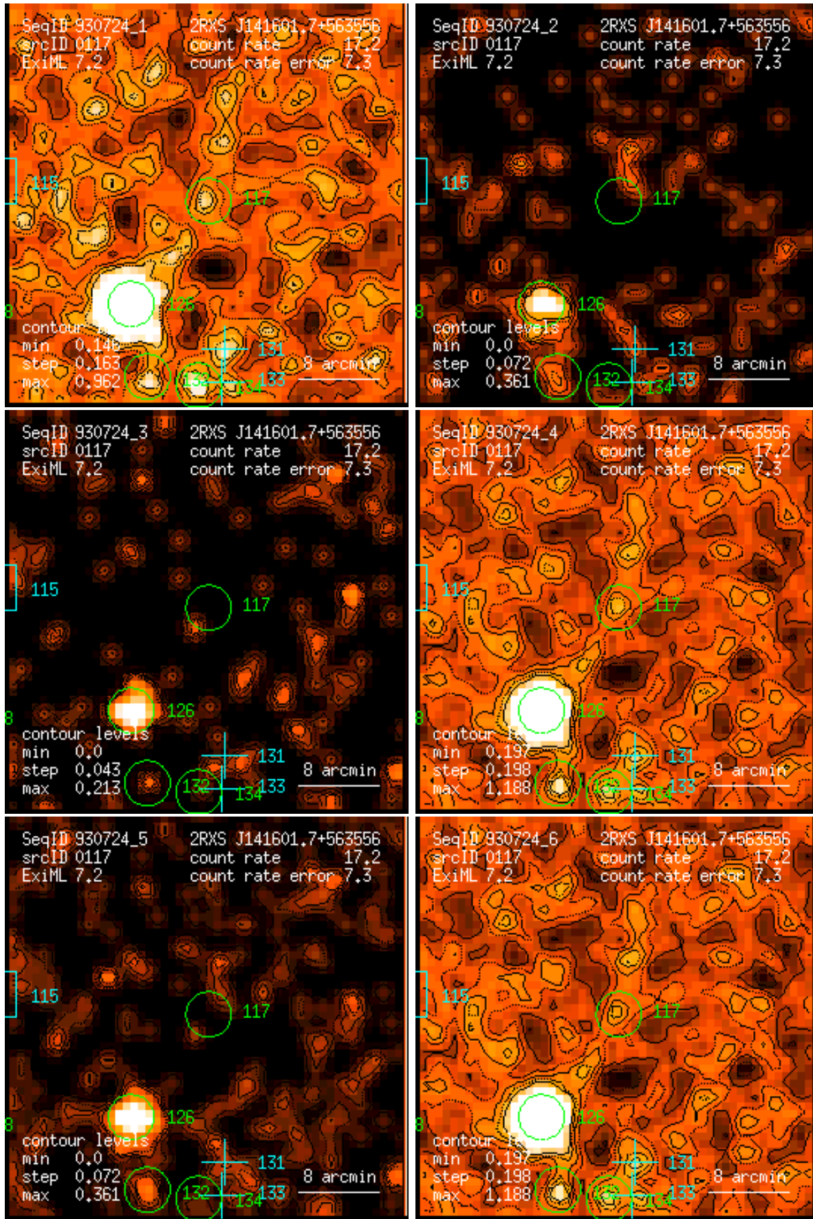
Figure 117: RASS 930724: detection 0117: band rate images, Gaussian filter: (1) PSPC channels 11 – 41, (2) 52 – 90, (3) 91 – 201, (4) 11 – 235, (5) 52 – 201, (6) 11 – 201. Broad band rates in counts/ks. Band rate contour levels in counts/ks/arcmin 2 .
