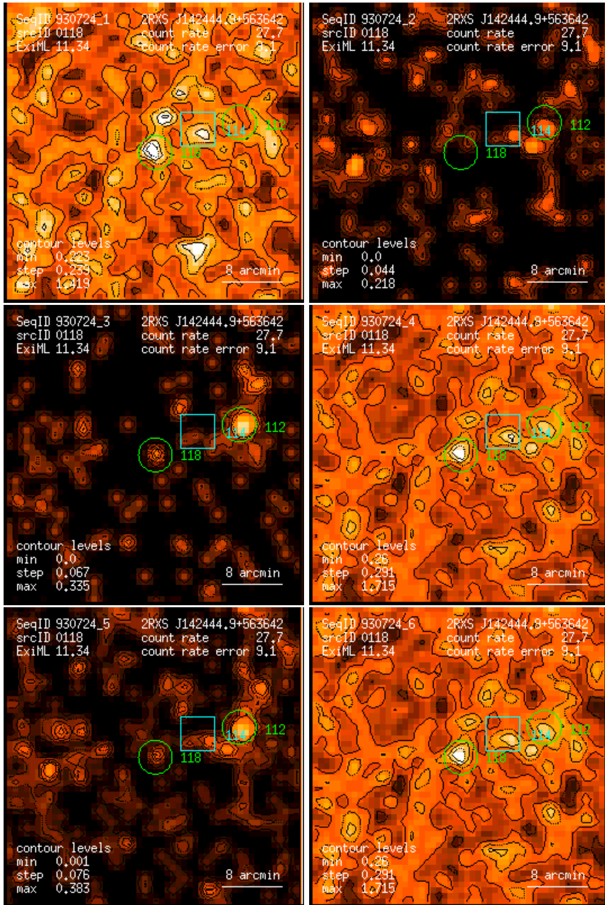
Figure 118: RASS 930724: detection 0118: band rate images, Gaussian filter: (1) PSPC channels 11 – 41, (2) 52 – 90, (3) 91 – 201, (4) 11 – 235, (5) 52 – 201, (6) 11 – 201. Broad band rates in counts/ks. Band rate contour levels in counts/ks/arcmin 2 .
