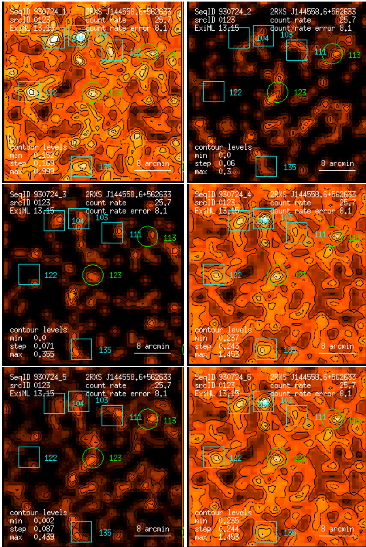
Figure 123: RASS 930724: detection 0123: band rate images, Gaussian filter: (1) PSPC channels 11 – 41, (2) 52 – 90, (3) 91 – 201, (4) 11 – 235, (5) 52 – 201, (6) 11 – 201. Broad band rates in counts/ks. Band rate contour levels in counts/ks/arcmin 2 .
