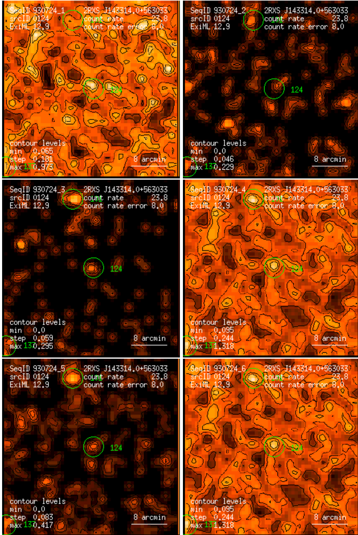
Figure 124: RASS 930724: detection 0124: band rate images, Gaussian filter: (1) PSPC channels 11 – 41, (2) 52 – 90, (3) 91 – 201, (4) 11 – 235, (5) 52 – 201, (6) 11 – 201. Broad band rates in counts/ks. Band rate contour levels in counts/ks/arcmin 2 .
