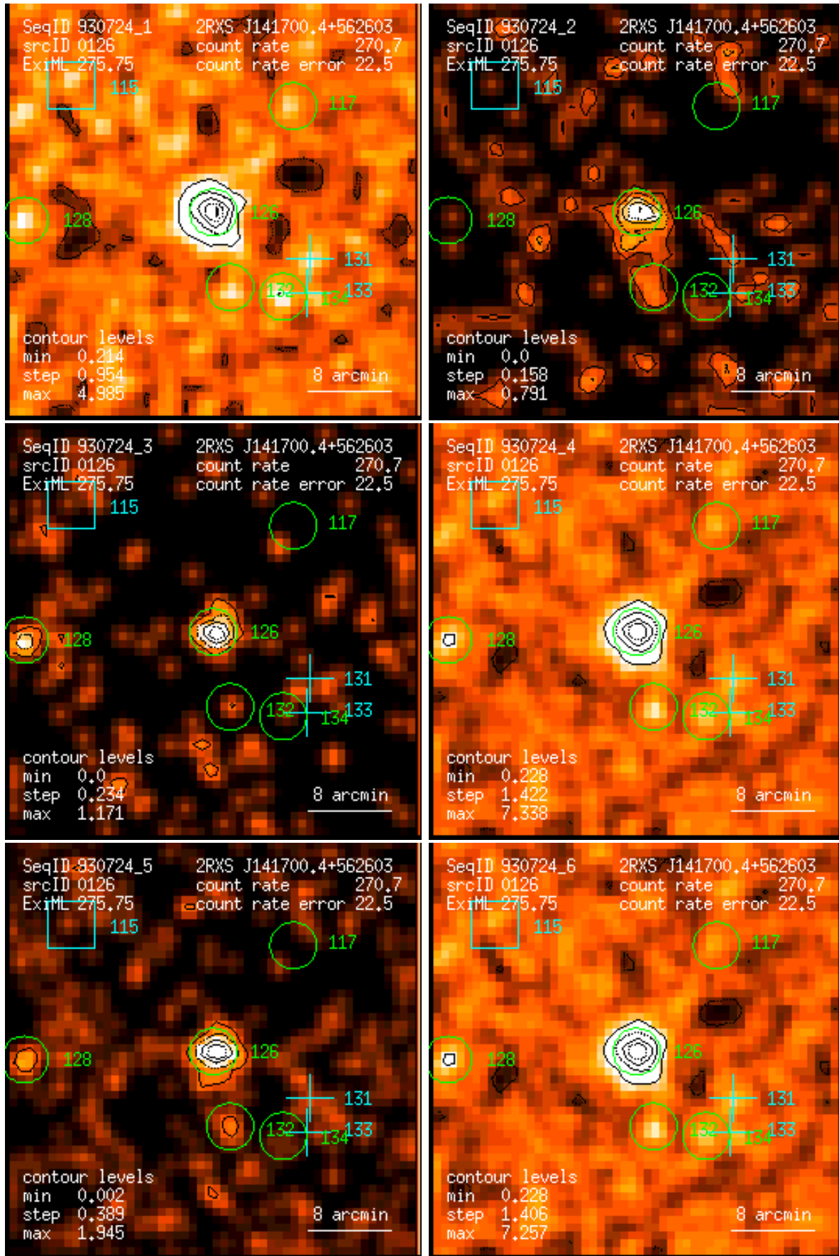
Figure 126: RASS 930724: detection 0126: band rate images, Gaussian filter: (1) PSPC channels 11 – 41, (2) 52 – 90, (3) 91 – 201, (4) 11 – 235, (5) 52 – 201, (6) 11 – 201. Broad band rates in counts/ks. Band rate contour levels in counts/ks/arcmin 2 .
