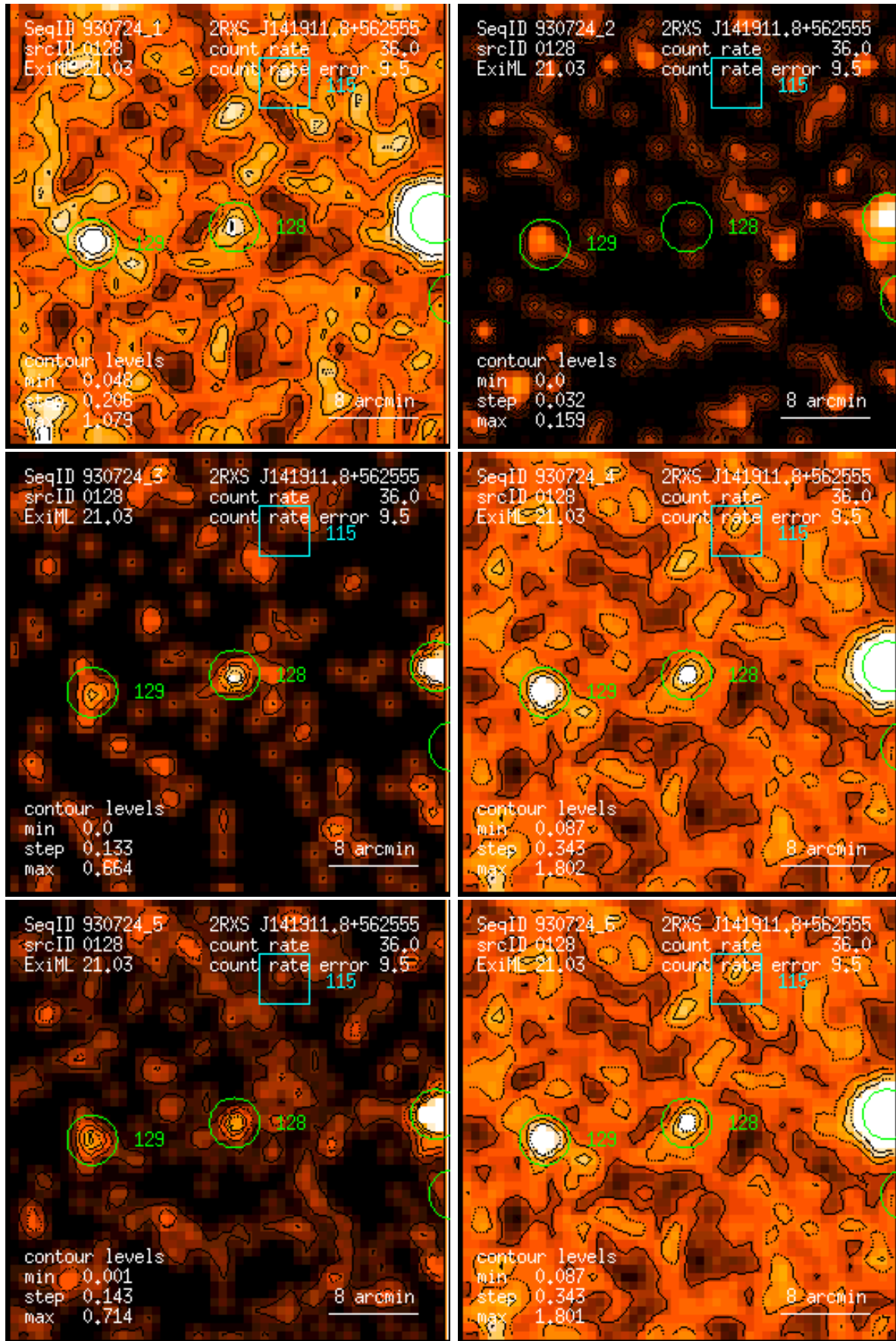
Figure 128: RASS 930724: detection 0128: band rate images, Gaussian filter: (1) PSPC channels 11 – 41, (2) 52 – 90, (3) 91 – 201, (4) 11 – 235, (5) 52 – 201, (6) 11 – 201. Broad band rates in counts/ks. Band rate contour levels in counts/ks/arcmin 2 .
