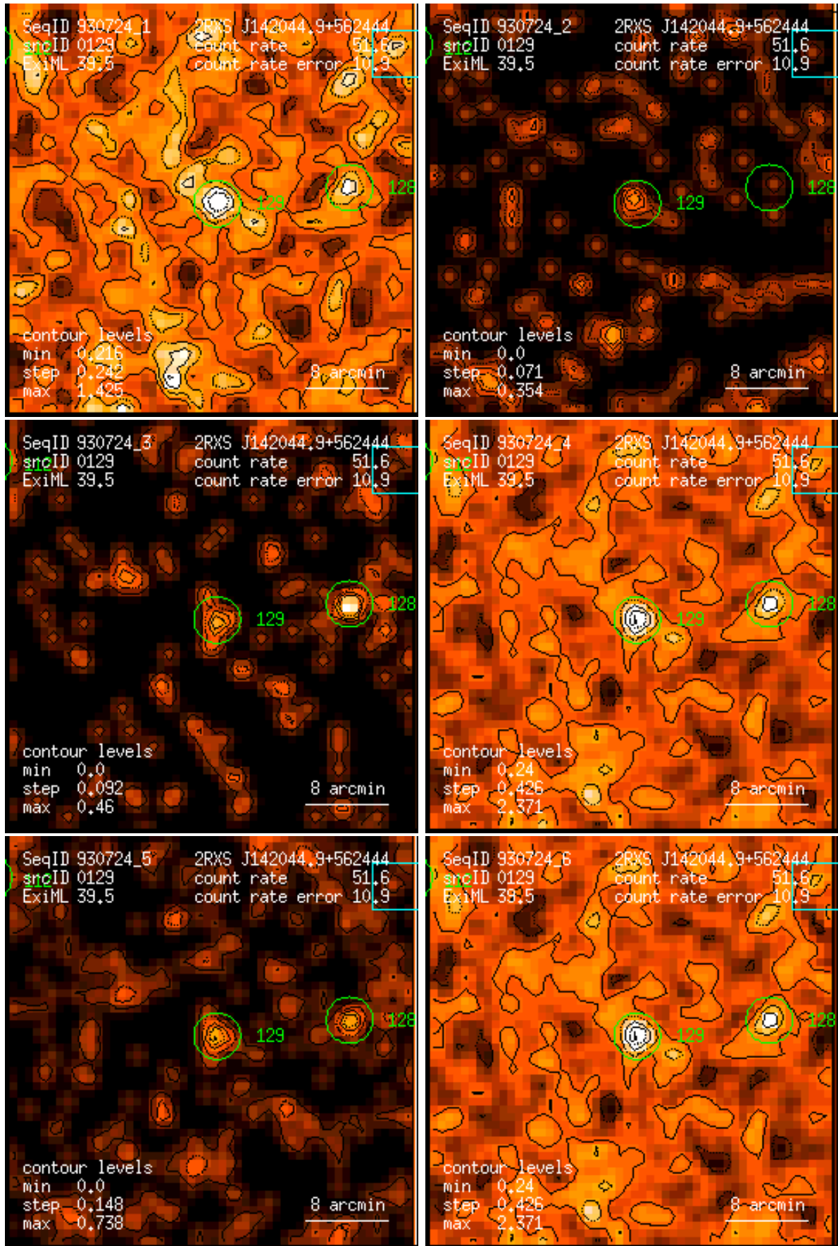
Figure 129: RASS 930724: detection 0129: band rate images, Gaussian filter: (1) PSPC channels 11 – 41, (2) 52 – 90, (3) 91 – 201, (4) 11 – 235, (5) 52 – 201, (6) 11 – 201. Broad band rates in counts/ks. Band rate contour levels in counts/ks/arcmin 2 .
