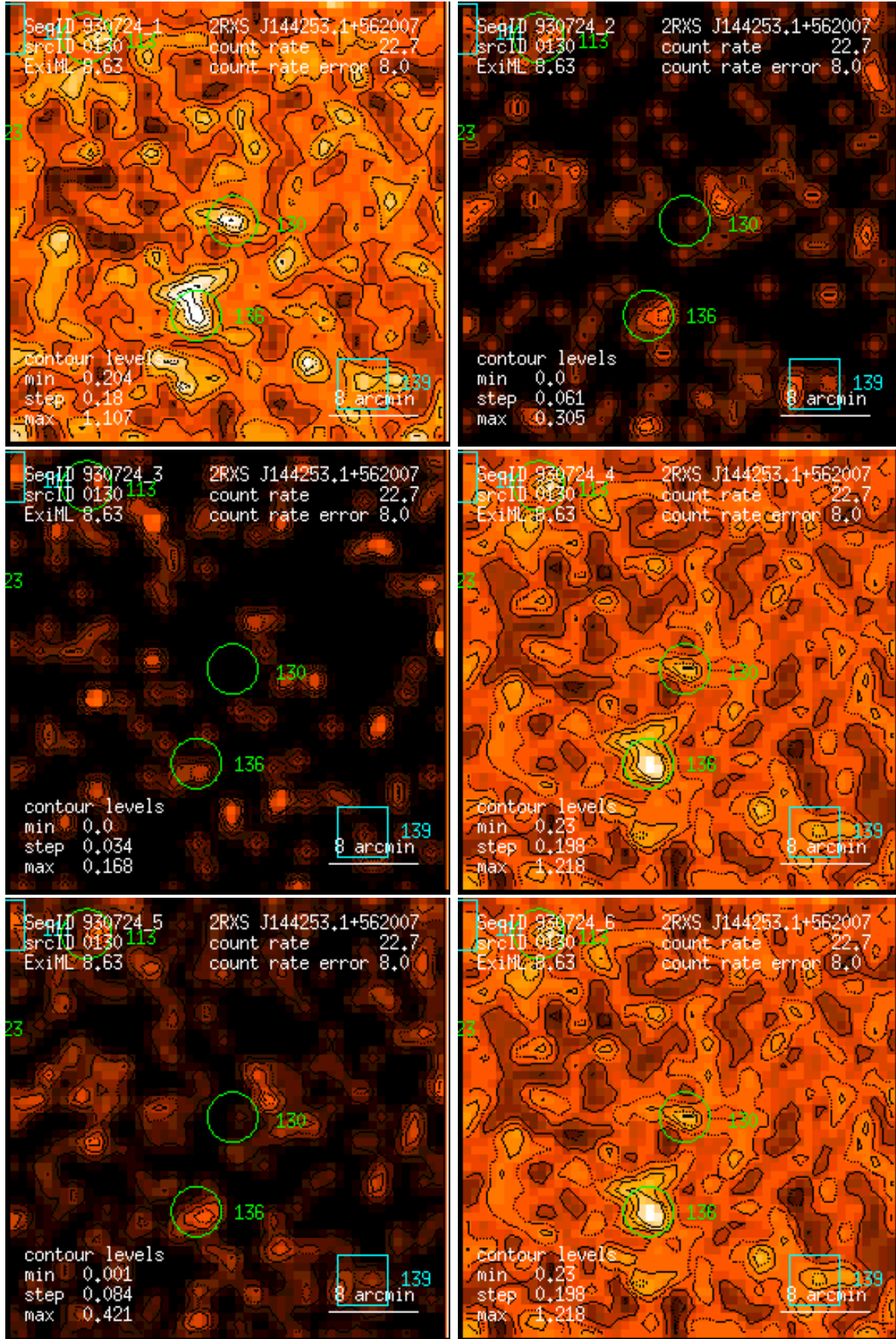
Figure 130: RASS 930724: detection 0130: band rate images, Gaussian filter: (1) PSPC channels 11 – 41, (2) 52 – 90, (3) 91 – 201, (4) 11 – 235, (5) 52 – 201, (6) 11 – 201. Broad band rates in counts/ks. Band rate contour levels in counts/ks/arcmin 2 .
