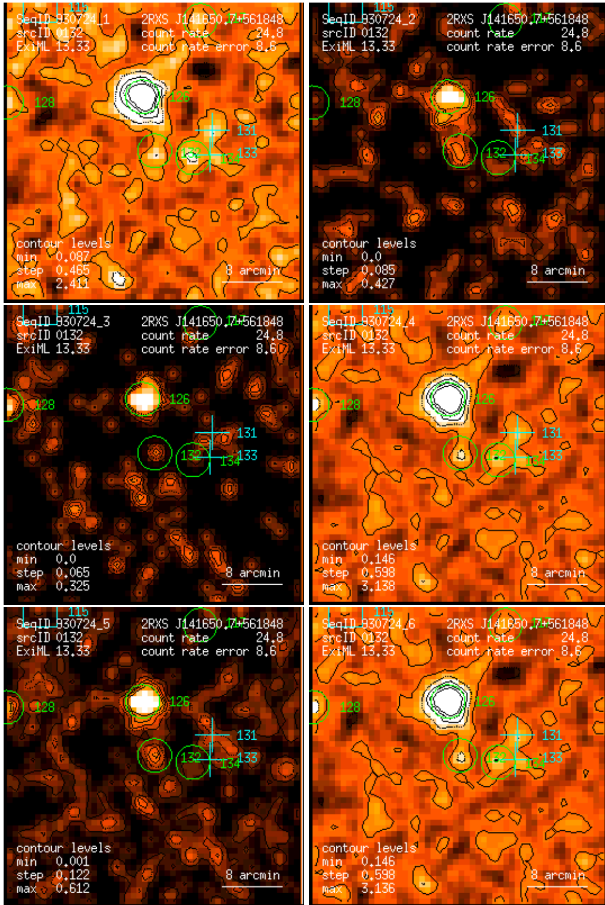
Figure 132: RASS 930724: detection 0132: band rate images, Gaussian filter: (1) PSPC channels 11 – 41, (2) 52 – 90, (3) 91 – 201, (4) 11 – 235, (5) 52 – 201, (6) 11 – 201. Broad band rates in counts/ks. Band rate contour levels in counts/ks/arcmin 2 .
