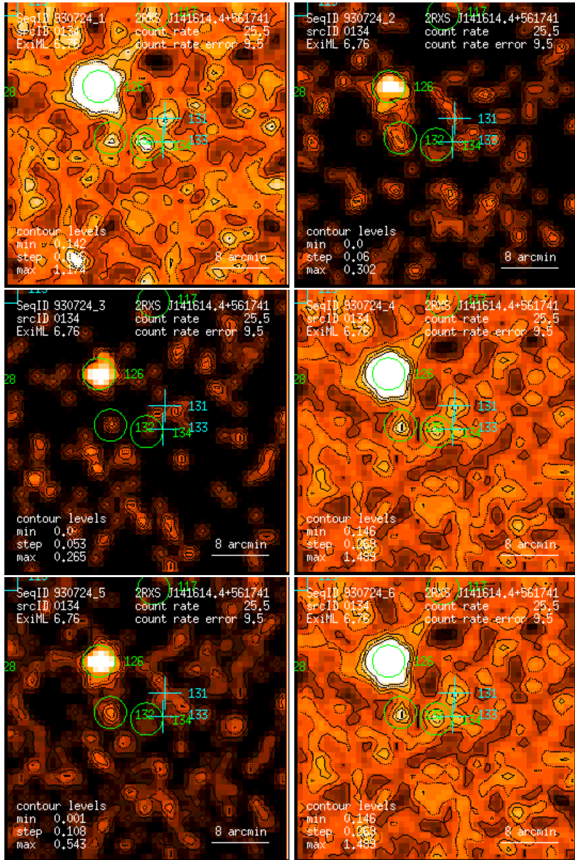
Figure 134: RASS 930724: detection 0134: band rate images, Gaussian filter: (1) PSPC channels 11 – 41, (2) 52 – 90, (3) 91 – 201, (4) 11 – 235, (5) 52 – 201, (6) 11 – 201. Broad band rates in counts/ks. Band rate contour levels in counts/ks/arcmin 2 .
