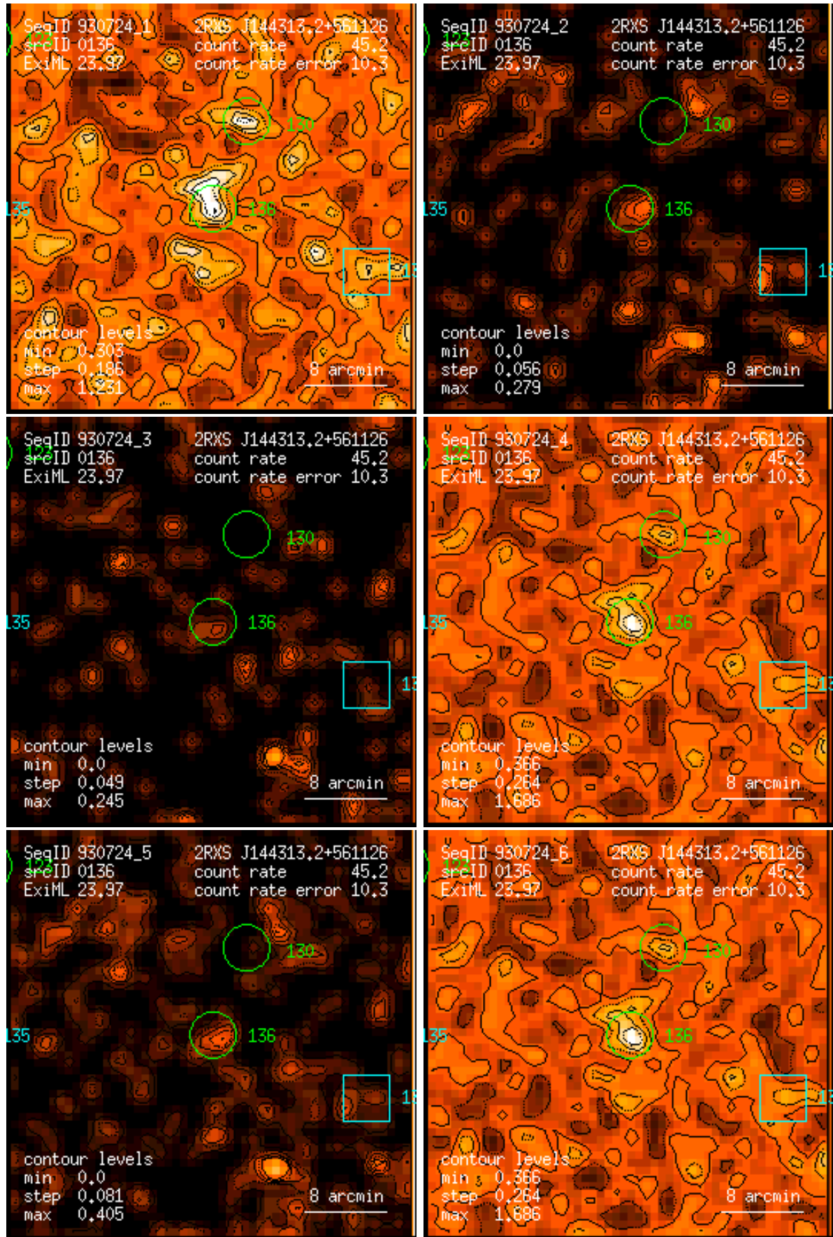
Figure 136: RASS 930724: detection 0136: band rate images, Gaussian filter: (1) PSPC channels 11 – 41, (2) 52 – 90, (3) 91 – 201, (4) 11 – 235, (5) 52 – 201, (6) 11 – 201. Broad band rates in counts/ks. Band rate contour levels in counts/ks/arcmin 2 .
