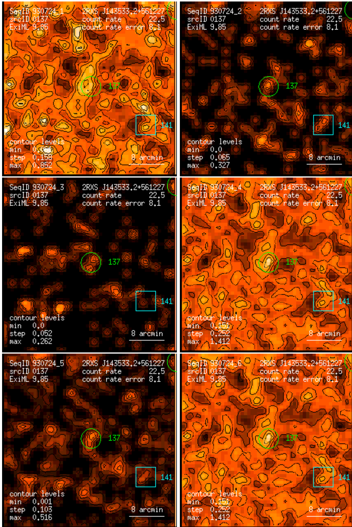
Figure 137: RASS 930724: detection 0137: band rate images, Gaussian filter: (1) PSPC channels 11 – 41, (2) 52 – 90, (3) 91 – 201, (4) 11 – 235, (5) 52 – 201, (6) 11 – 201. Broad band rates in counts/ks. Band rate contour levels in counts/ks/arcmin 2 .
