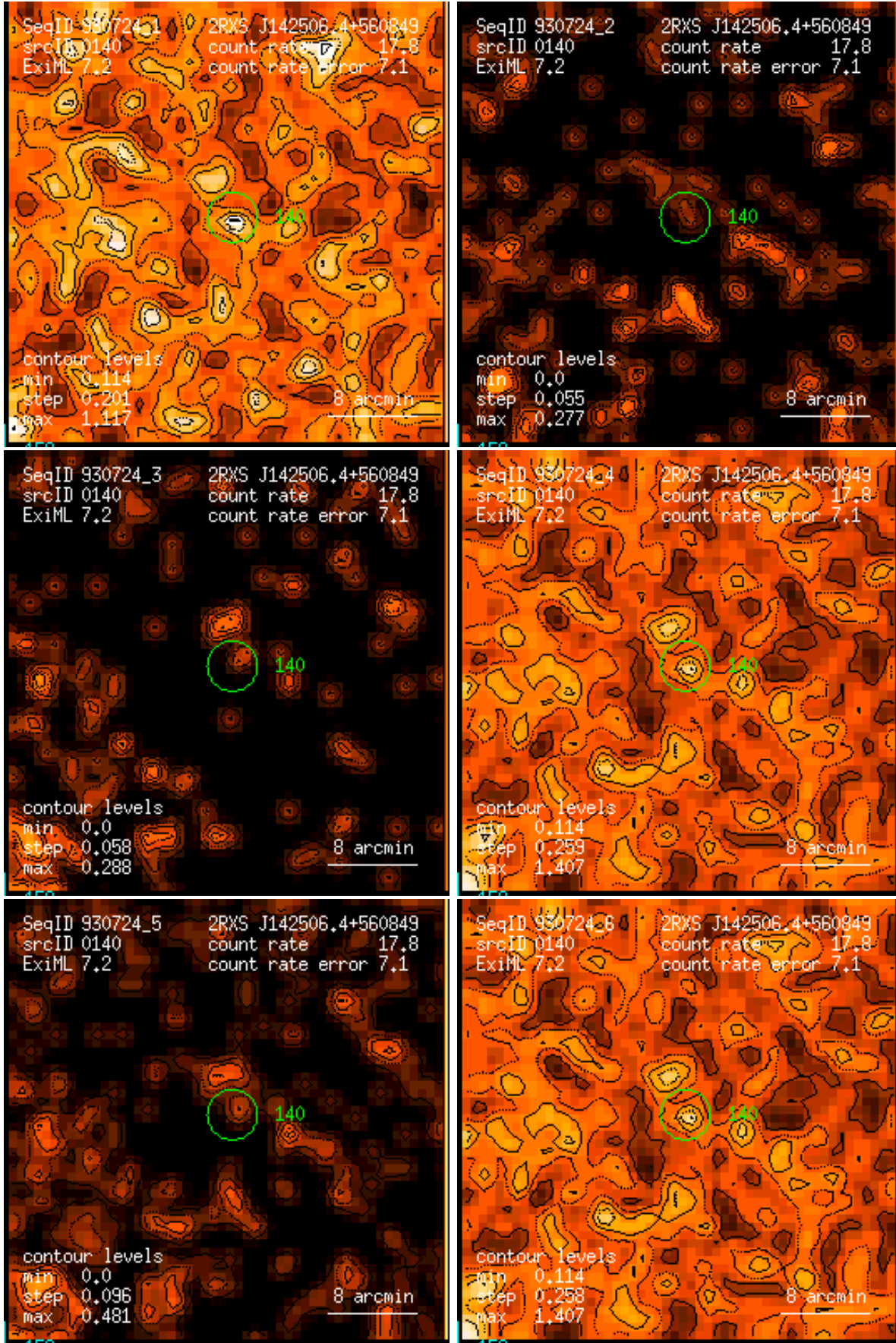
Figure 140: RASS 930724: detection 0140: band rate images, Gaussian filter: (1) PSPC channels 11 – 41, (2) 52 – 90, (3) 91 – 201, (4) 11 – 235, (5) 52 – 201, (6) 11 – 201. Broad band rates in counts/ks. Band rate contour levels in counts/ks/arcmin 2 .
