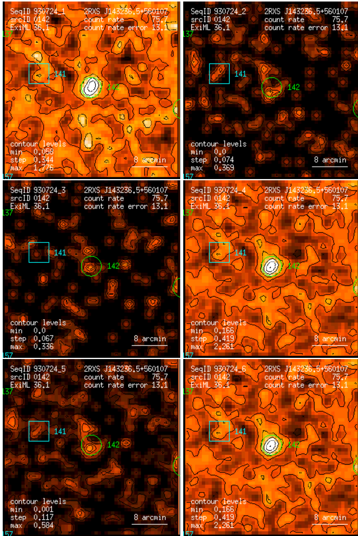
Figure 142: RASS 930724: detection 0142: band rate images, Gaussian filter: (1) PSPC channels 11 – 41, (2) 52 – 90, (3) 91 – 201, (4) 11 – 235, (5) 52 – 201, (6) 11 – 201. Broad band rates in counts/ks. Band rate contour levels in counts/ks/arcmin 2 .
