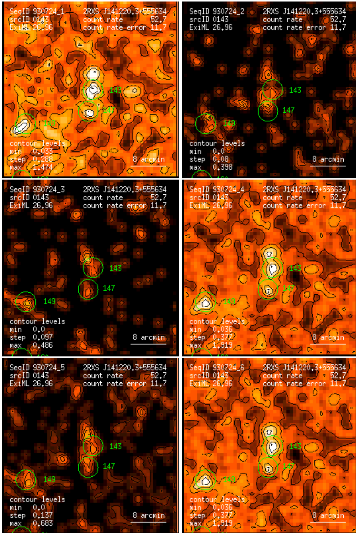
Figure 143: RASS 930724: detection 0143: band rate images, Gaussian filter: (1) PSPC channels 11 – 41, (2) 52 – 90, (3) 91 – 201, (4) 11 – 235, (5) 52 – 201, (6) 11 – 201. Broad band rates in counts/ks. Band rate contour levels in counts/ks/arcmin 2 .
